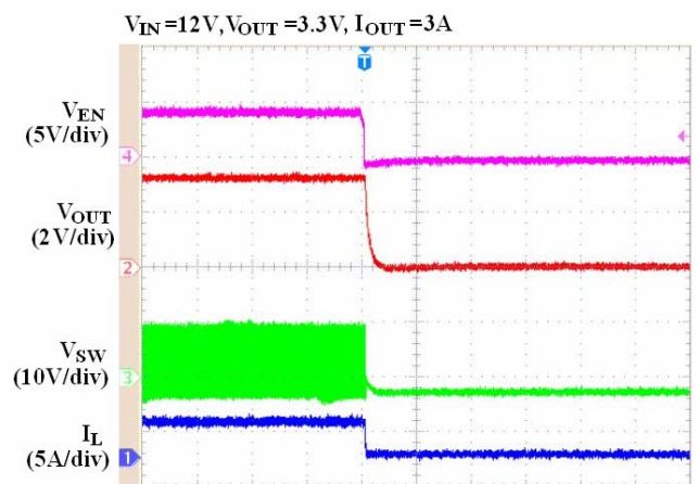
Times (200us/div)
