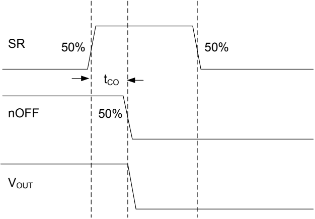
图 12. Timing Diagram (nSR0 + nOFF vs. V OUT ) 2
