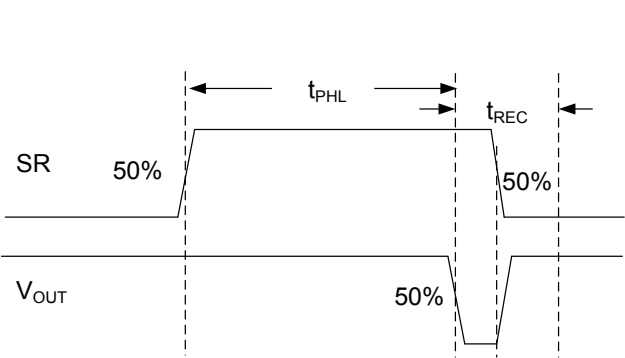
图 7. Power-On with SR
