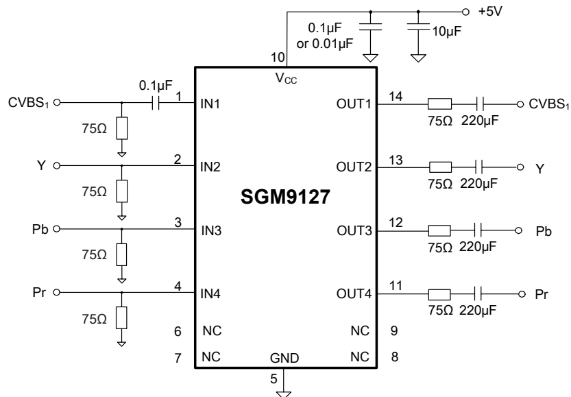
Figure 1. AC Coupling Application Schematic
