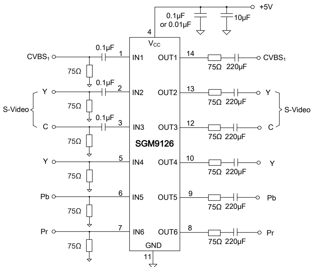
Figure 1. AC Coupling Application Schematic
