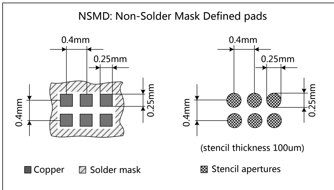
Figure 34. Footprint
