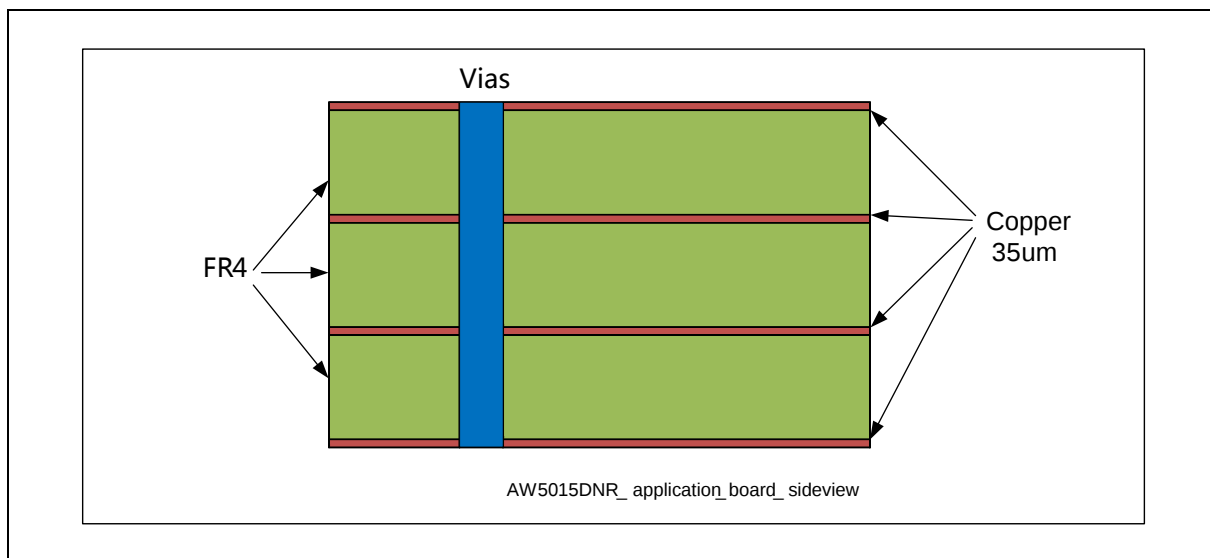
Figure 26. Drawing of Application Board
