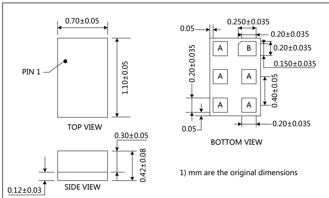
Figure 32. Package Outline
