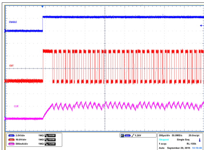
Figure 8. DRV8828 Current Limiting
