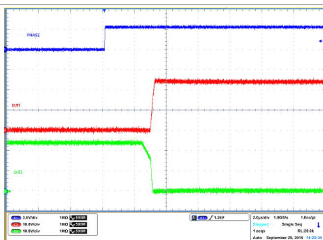
Figure 9. DRV8828 Direction Change
