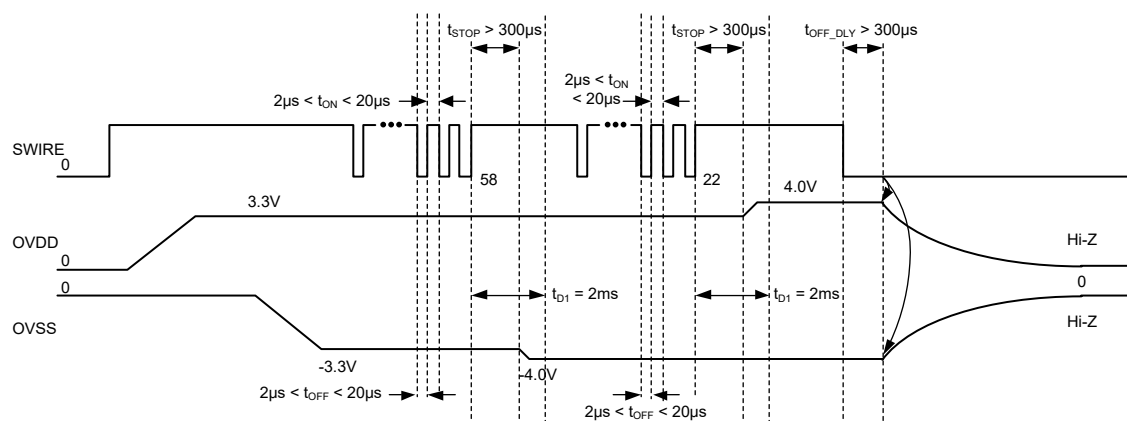
SWIRE Command Timing Diagram
