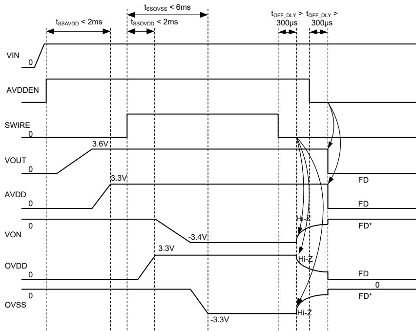
Figure 2. Startup and Shutdown Sequence 1 (FD= Fast Discharge, FD*= Fast Discharge for 30ms)
