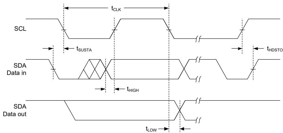
Figure 2. Timing Diagram
