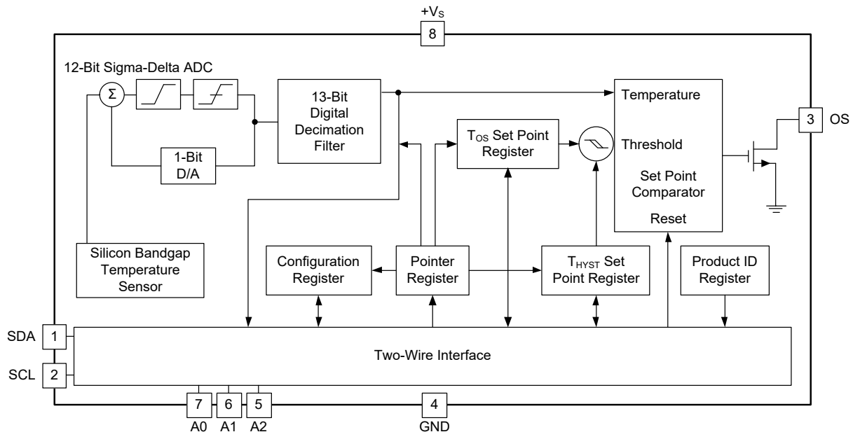
Figure 5. Block Diagram
