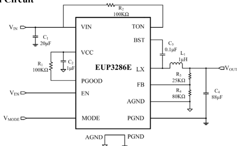
Figure 1. Application Circuit
