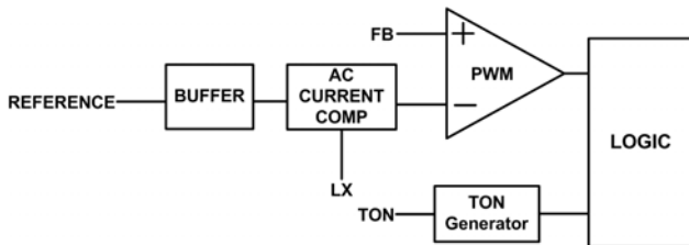
Figure 3. Simplified control topology of EUP3286E
