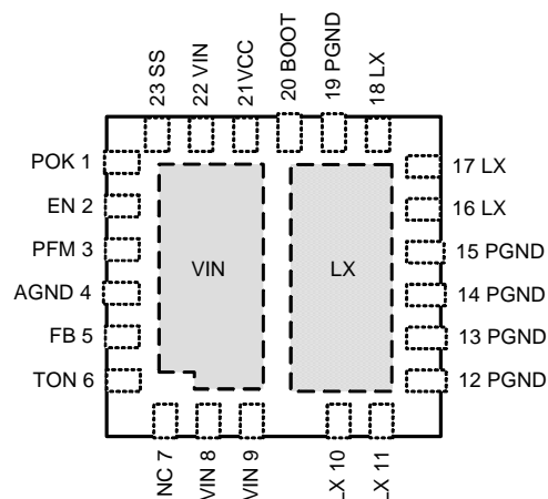
TQFN 4x4 -23 (TOP VIEW)
