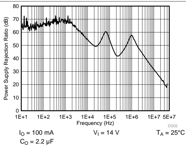
Figure 8. Power Supply Rejection Ratio
