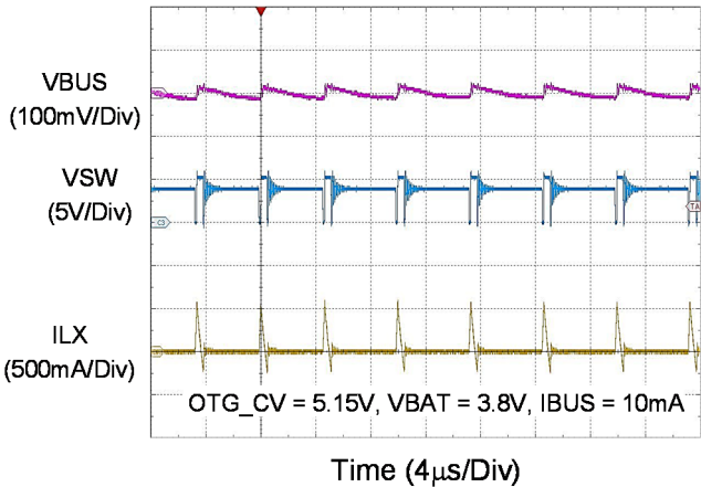
Boost Switching
