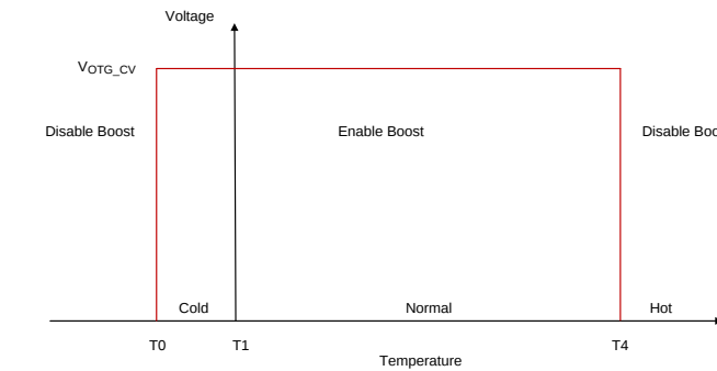
Figure 7. Thermal Protect During Boost Mode
