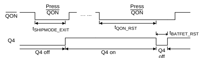
Figure 2. \overline{\text{QON}} Timing
