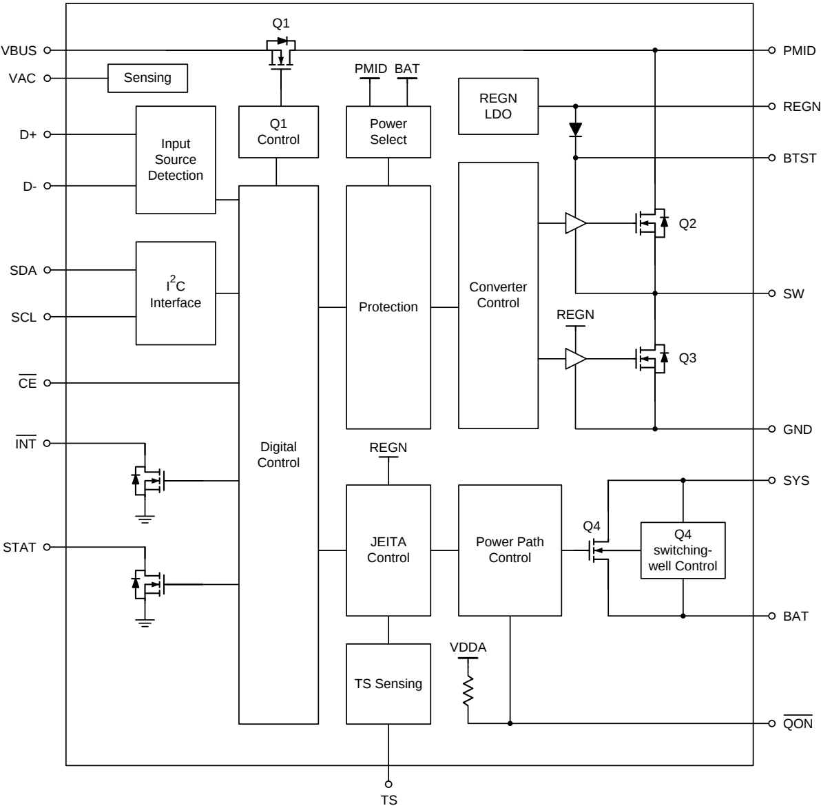
RT9471D Functional Block Diagram
