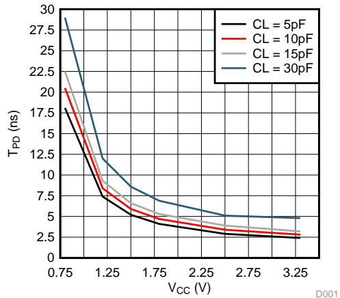
Figure 1. Propagation Delay vs. Supply Voltage and Load Capacitance
