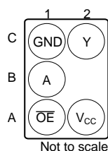
YZP or YZT Package 5-Pin DSBGA Bottom View
