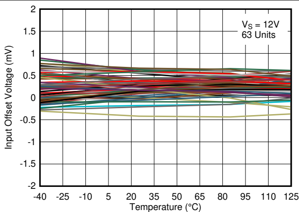
Figure 6-20. Input Offset Voltage vs. Temperature at 12\text{ V}
