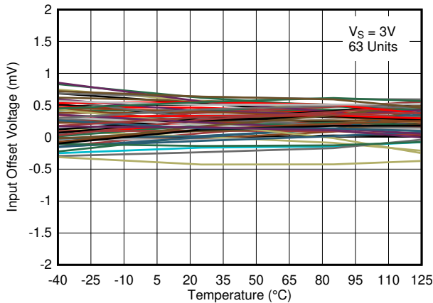
Figure 6-18. Input Offset Voltage vs. Temperature at 3\text{ V}
