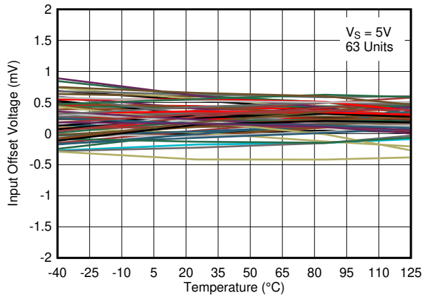
Figure 6-19. Input Offset Voltage vs. Temperature at 5\text{ V}
