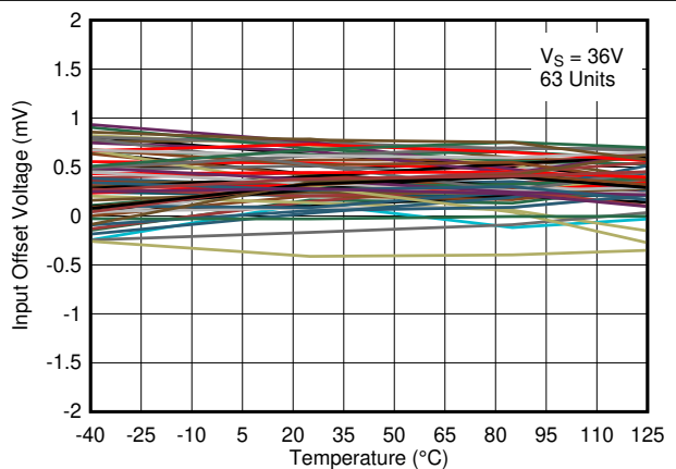
Figure 6-21. Input Offset Voltage vs. Temperature at 36\text{ V}
