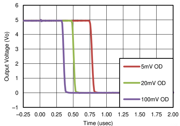
Figure 8-3. Response Time for Various Overdrives (Negative Transition)
