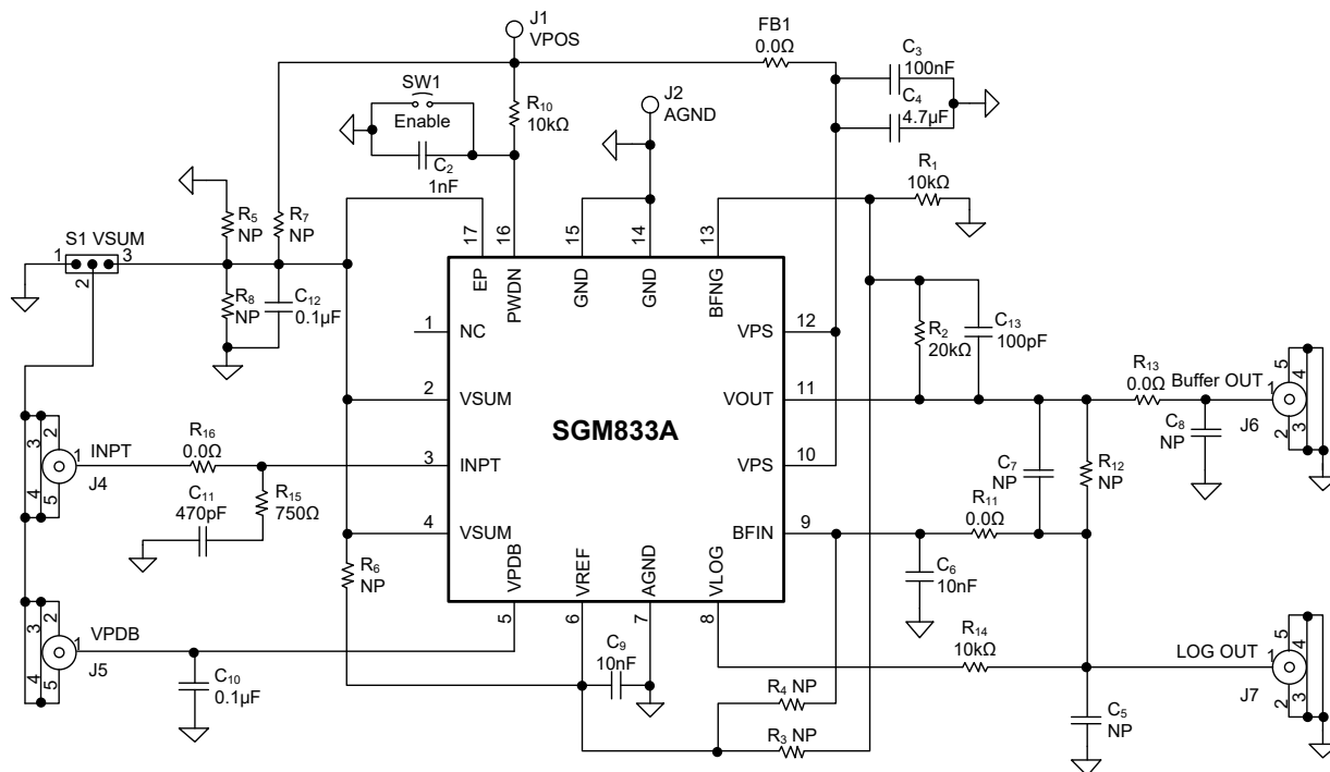
Some starting points for selecting the filter components for a few gain (G) examples and 1kHz cut-off frequency are provided in Table 3. The cut-off frequency can be increased or decreased by scaling the capacitor values.
