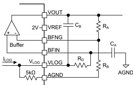
Some starting points for selecting the filter components for a few gain (G) examples and 1kHz cut-off frequency are provided in Table 3. The cut-off frequency can be increased or decreased by scaling the capacitor values.
