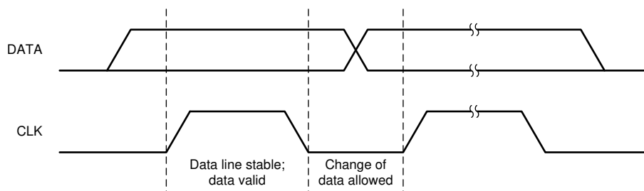
图 21. Bit Transfer on the Serial Interface
