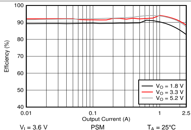
图 32. Efficiency versus Output Current
