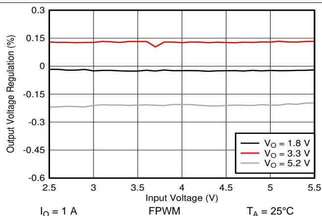
图 35. Line Regulation
