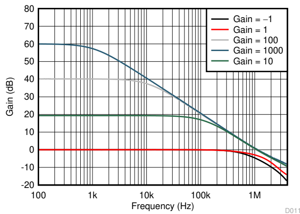
Figure 7-11. Closed-Loop Gain vs Frequency
