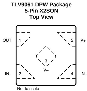
Pin Functions: TLV9061
