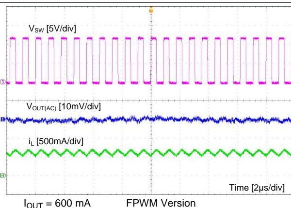
图 20. Ripple at Full Load
