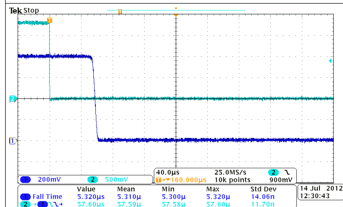
Figure 27. Turnoff Response Time (V_{IN} = 0.8\text{ V}, V_{BIAS} = 2.5\text{ V}, C_{IN} = 1\text{ μF}, C_L = 0.1\text{ μF}, R_L = 10\text{ Ω}) CH1: VOUT, CH2: ON
