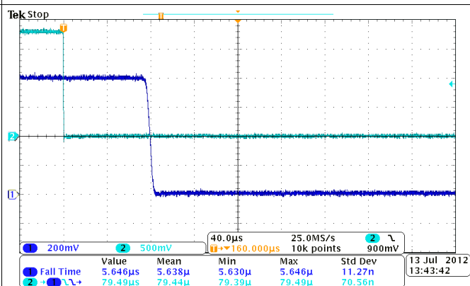
Figure 28. Turnoff Response Time (V_{IN} = 0.8\text{ V}, V_{BIAS} = 5\text{ V}, C_{IN} = 1\text{ μF}, C_L = 0.1\text{ μF}, R_L = 10\text{ Ω}) CH1: VOUT, CH2: ON
