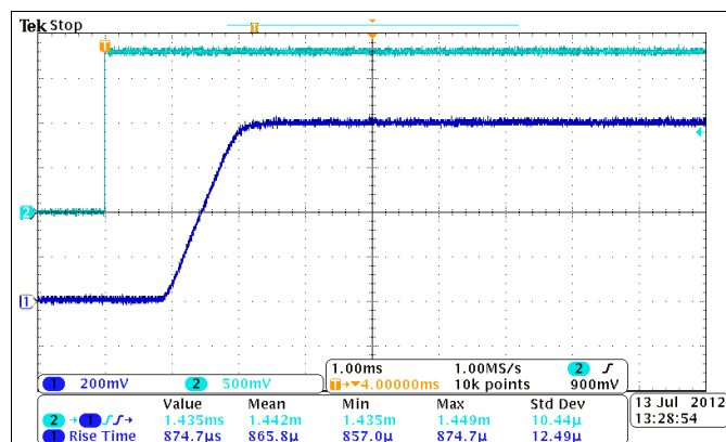
Figure 23. Turnon Response Time (V_{IN} = 0.8\text{ V}, V_{BIAS} = 2.5\text{ V}, C_{IN} = 1\text{ μF}, C_L = 0.1\text{ μF}, R_L = 10\text{ Ω}) CH1: VOUT, CH2: ON
