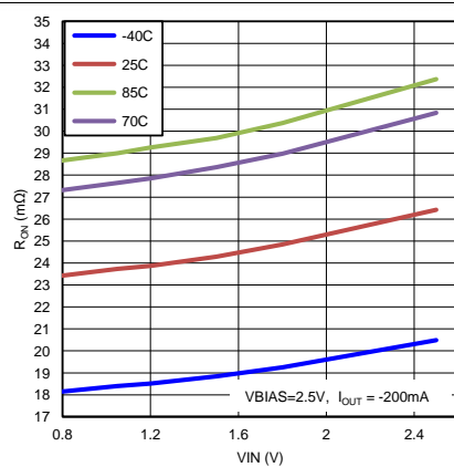
Figure 7. V_{IN} vs R_{ON} ( V_{BIAS} = 2.5\text{ V} )
