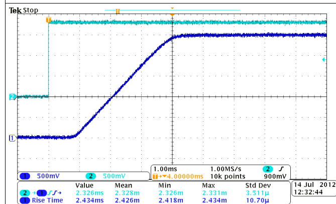
Figure 25. Turnon Response Time (V_{IN} = 2.5\text{ V}, V_{BIAS} = 2.5\text{ V}, C_{IN} = 1\text{ μF}, C_L = 0.1\text{ μF}, R_L = 10\text{ Ω}) CH1: VOUT, CH2: ON
