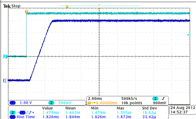
Figure 26. Turnon Response Time (V_{IN} = 5\text{ V}, V_{BIAS} = 5\text{ V}, C_{IN} = 1\text{ μF}, C_L = 0.1\text{ μF}, R_L = 10\text{ Ω}) CH1: VOUT, CH2: ON
