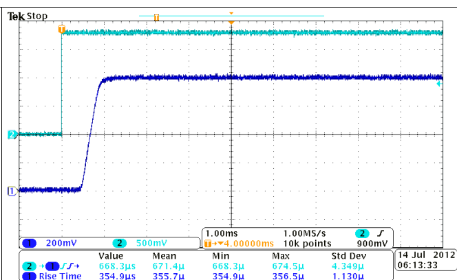
Figure 24. Turnon Response Time (V_{IN} = 0.8\text{ V}, V_{BIAS} = 5\text{ V}, C_{IN} = 1\text{ μF}, C_L = 0.1\text{ μF}, R_L = 10\text{ Ω}) CH1: VOUT, CH2: ON
