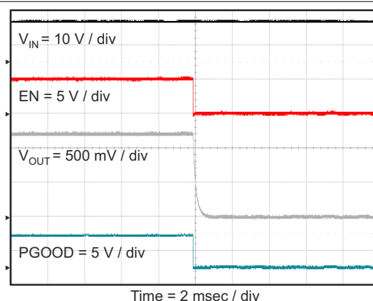
Figure 8-17. Shut Down Relative to EN Falling
