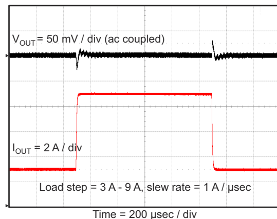
Figure 8-18. Transient Response
