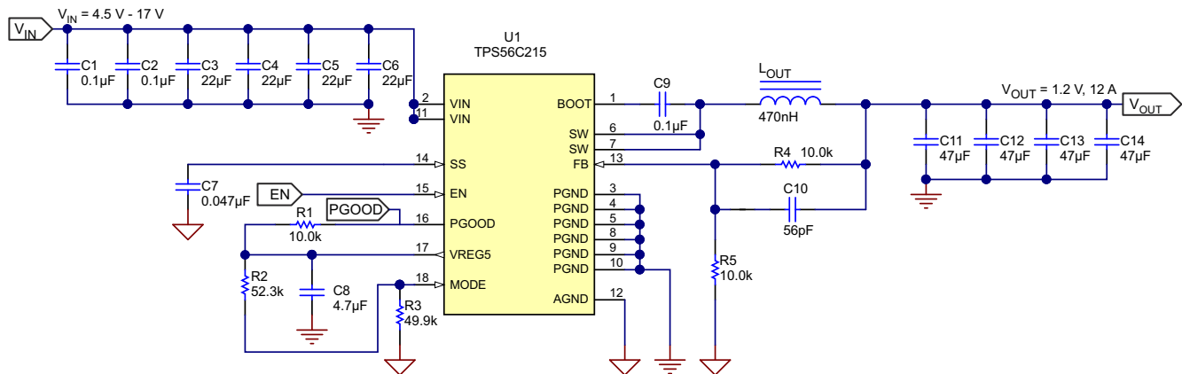
Figure 8-1. Application Schematic
