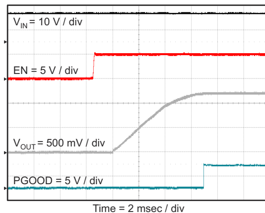
Figure 8-15. Start Up Relative to EN Rising
