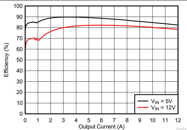
Figure 8-2. Efficiency
