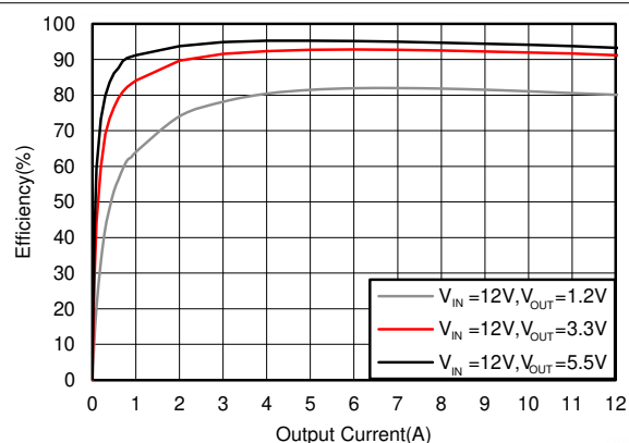
Figure 6-16. Efficiency, Mode = FCCM, F_{SW} = 1200 kHz
