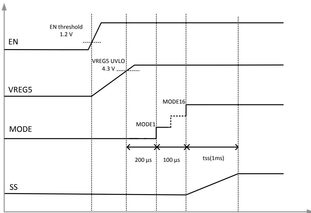
Figure 7-2. Power-Up Sequence
