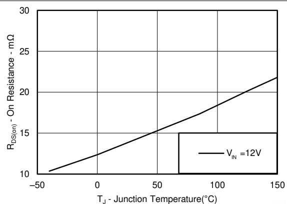
Figure 6-4. High-side R DS(on) vs Temperature
