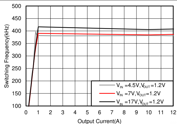
Figure 6-18. F_{SW} Load Regulation, Mode = DCM, F_{SW} = 400 kHz
