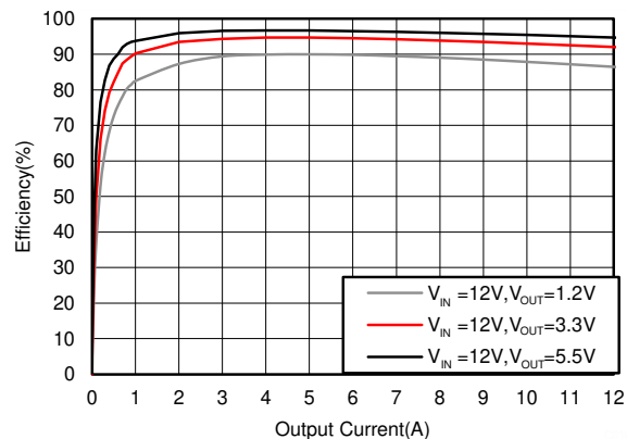
Figure 6-14. Efficiency, Mode = FCCM, F_{SW} = 400 kHz
