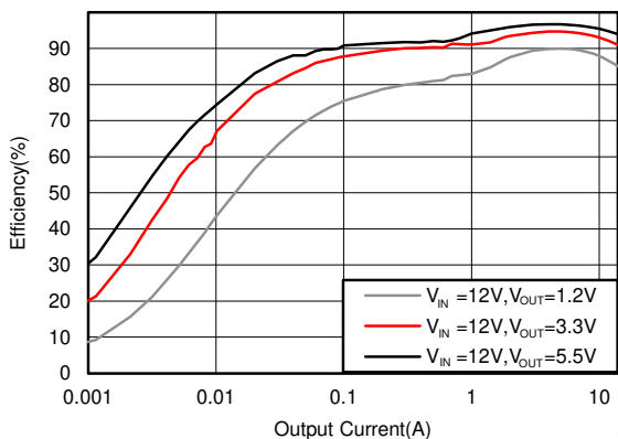
Figure 6-13. Efficiency, Mode = DCM, F_{SW} = 400 kHz
