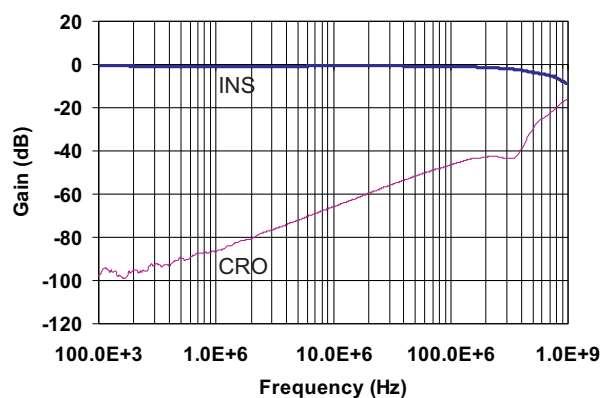
Figure 3. Crosstalk and Insertion Loss vs Frequency ( V_{CC} = 3\text{ V} )
