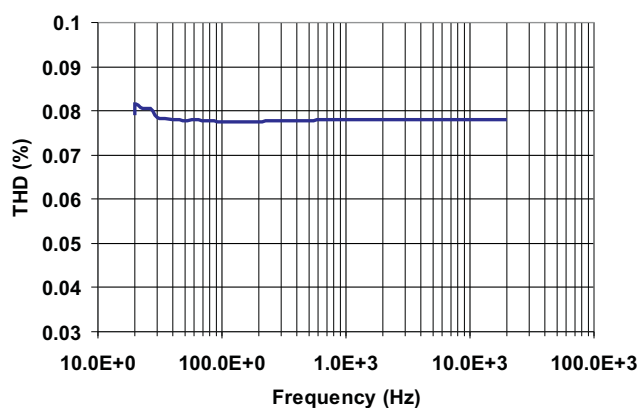
Figure 4. Total Harmonic Distortion vs Frequency
