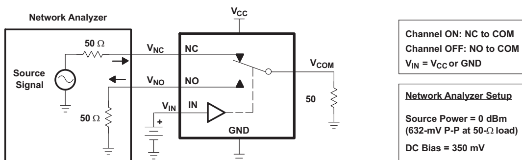
Figure 13. Crosstalk
