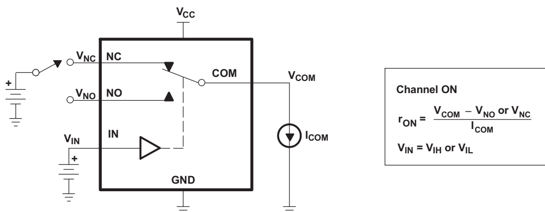
Figure 5. ON-State Resistance
