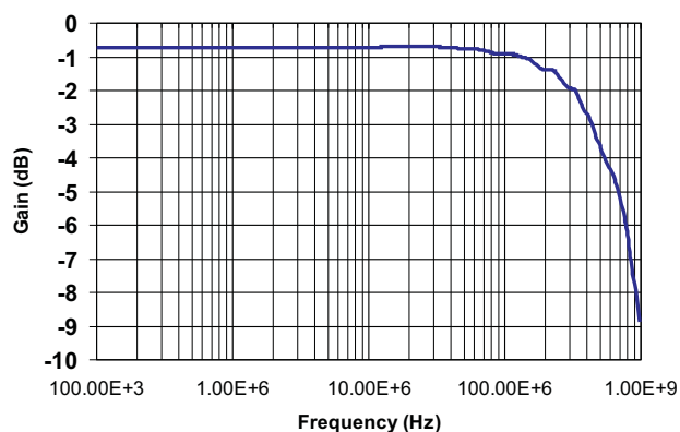
Figure 2. Bandwidth ( V_{CC} = 3\text{ V} )
