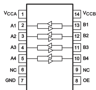
Figure 5-4. D or PW Package, 14-Pin SOIC or TSSOP (Top View)
