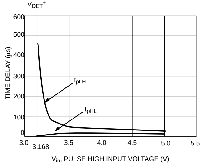
Figure 25. t_{pLH} and t_{pHL} vs. Input Voltage for the NCP301SNT1
