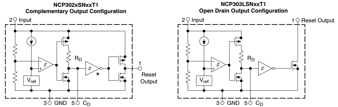
This device contains 28 active transistors. Figure 1. Representative Block Diagrams
