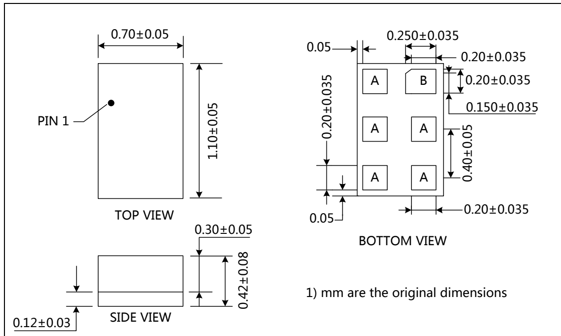
Figure 32. Package Outline
