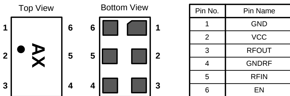
Figure 1. AW5025 Pin Configuration and Marking
