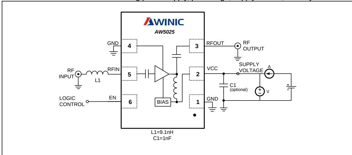
Figure 28. Circuit for DC test
