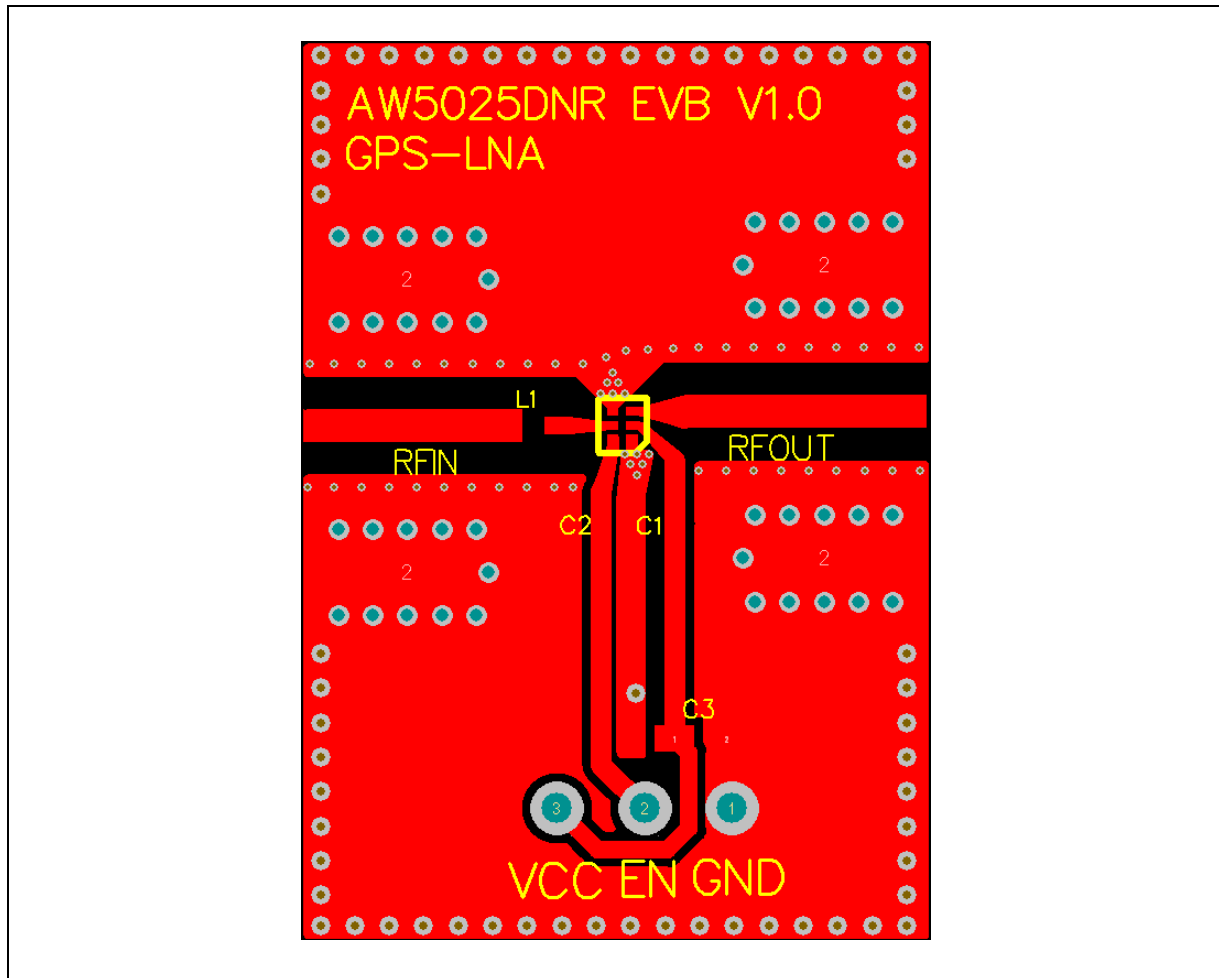
Figure 26. Drawing of Application Board
