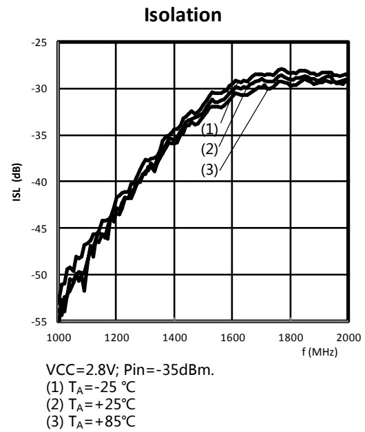
Figure 24. Isolation as a function of frequency; typical values
