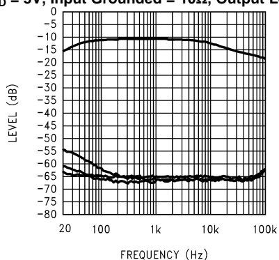
Figure 36. Top Trace = No Cap, Next Trace Down = 1μf Next Trace Down = 2μf, Bottom Trace = 4.7μf
