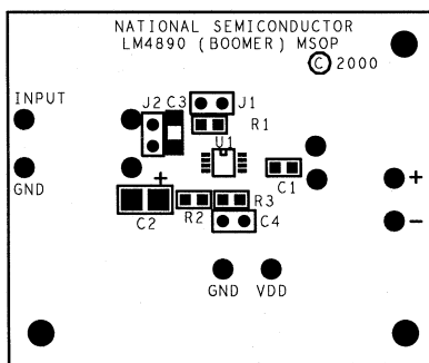
Figure 76. Top Layer
