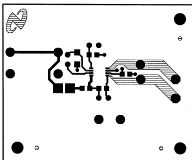
Figure 77. Bottom Layer
