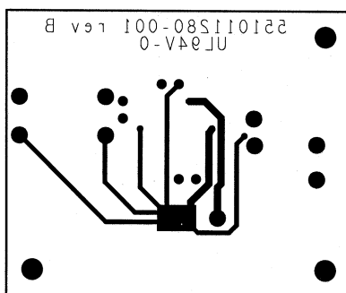
Figure 77. Bottom Layer
