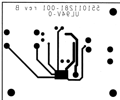
Figure 74. Bottom Layer
