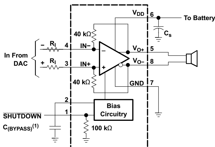
Figure 16. Typical Differential Input Application Schematic
