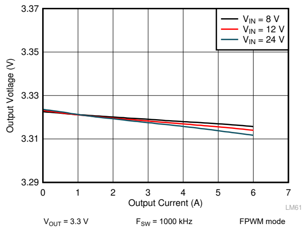
Figure 9-20. LM61460 Load and Line Regulation
