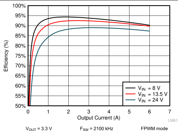
Figure 9-10. LM61460 Efficiency
