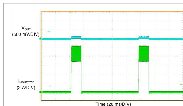
Figure 8-14. Inductor Current Bursts During Hiccup
