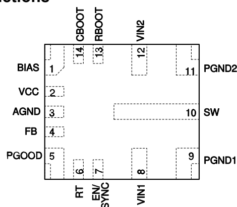
Figure 6-1. 14-Pin VQFN-HR RJR Package (Top View)
