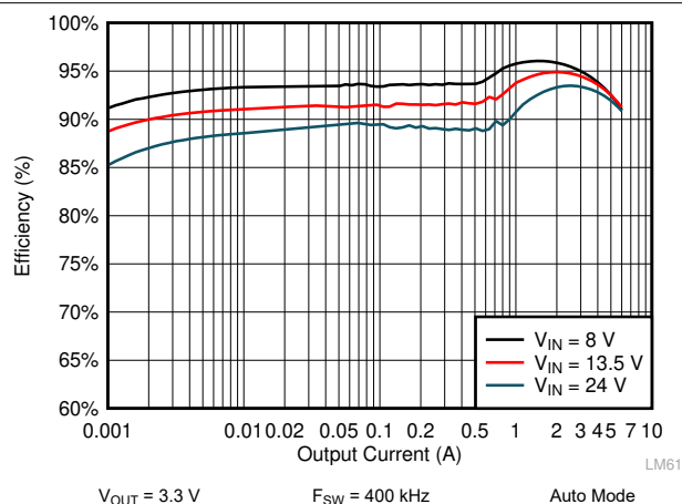
Figure 9-5. LM61460 Efficiency
