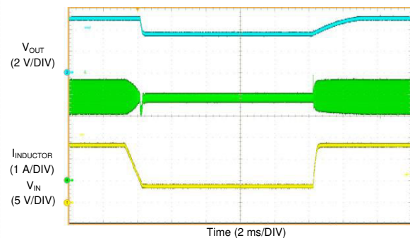
Figure 9-43. LM61460 Short Circuit Recovery
