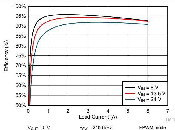
Figure 9-16. LM61460 Efficiency
