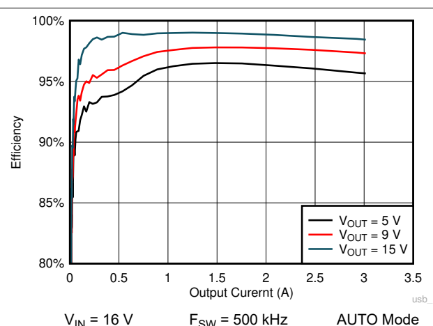
Figure 9-67. LM61460 Efficiency
