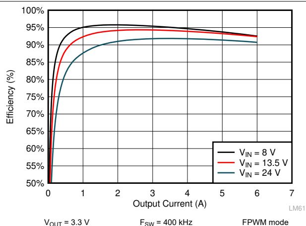
Figure 9-6. LM61460 Efficiency
