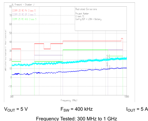
Figure 9-60. Radiated EMI Log Horizontal versus CISPR25 Limits
