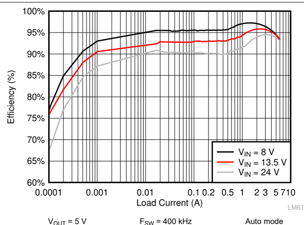
Figure 9-11. LM61460 Efficiency
