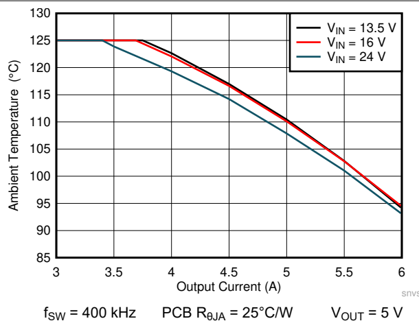
Figure 9-2. Maximum Ambient Temperature Versus Output Current
