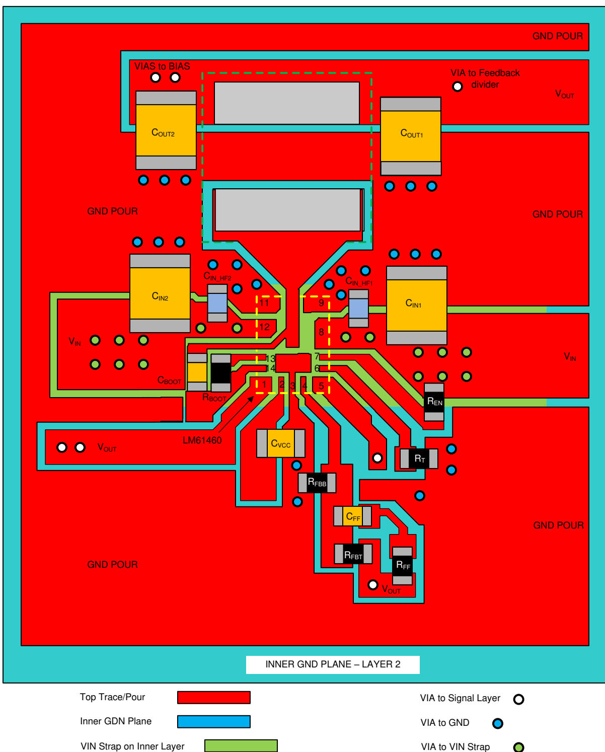
Figure 11-2. Layout Example
