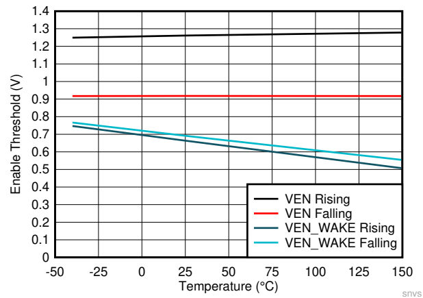
Figure 7-7. Enable Thresholds
