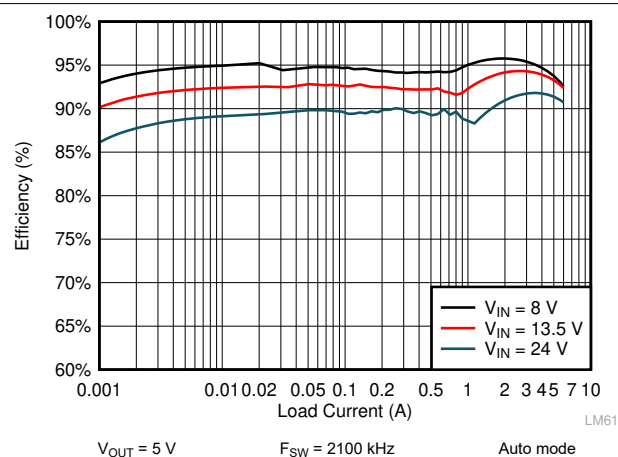
Figure 9-15. LM61460 Efficiency
