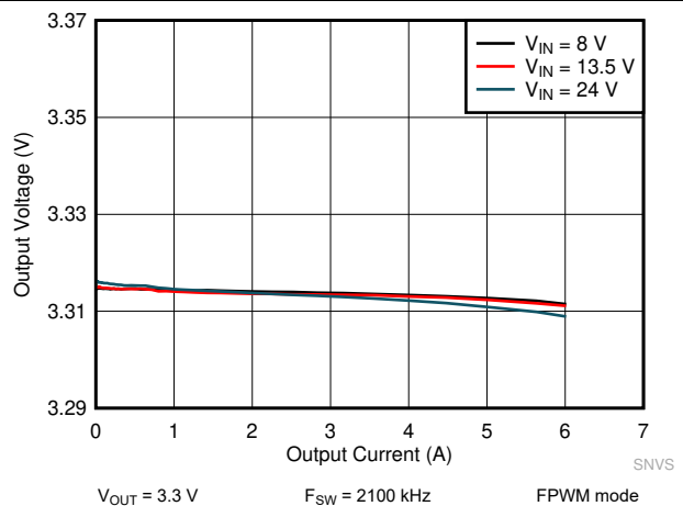
Figure 9-22. LM61460 Load and Line Regulation
