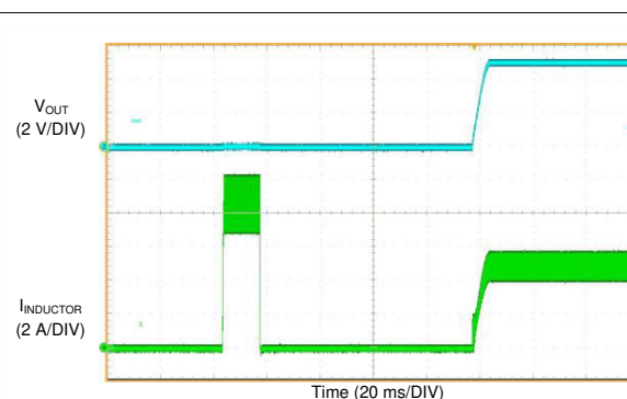
Figure 8-15. Short-Circuit Recovery
