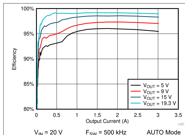
Figure 9-66. LM61460 Efficiency
