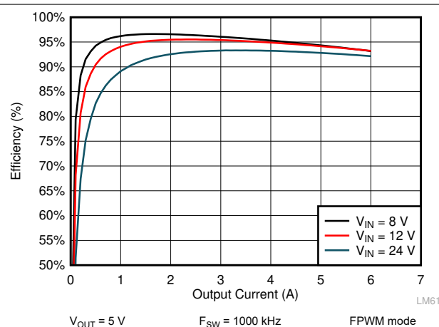
Figure 9-14. LM61460 Efficiency
