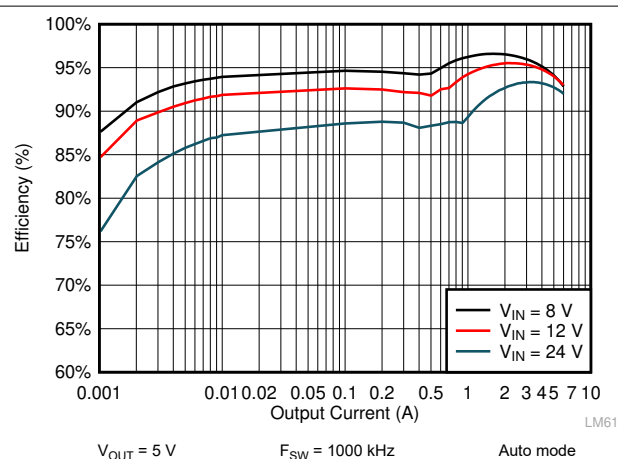
Figure 9-13. LM61460 Efficiency
