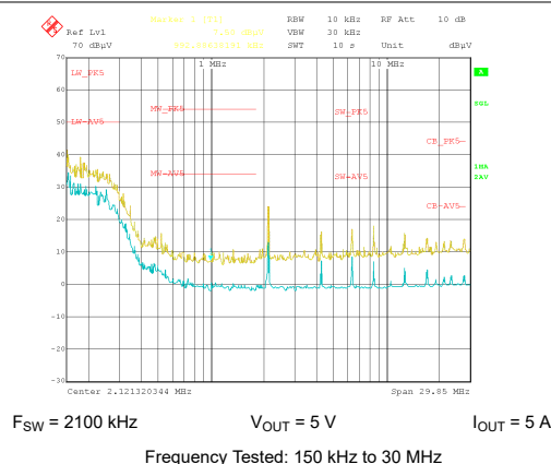
Figure 9-62. Conducted EMI versus CISPR25 Limits (Yellow: Peak Signal, Blue: Average Signal)
