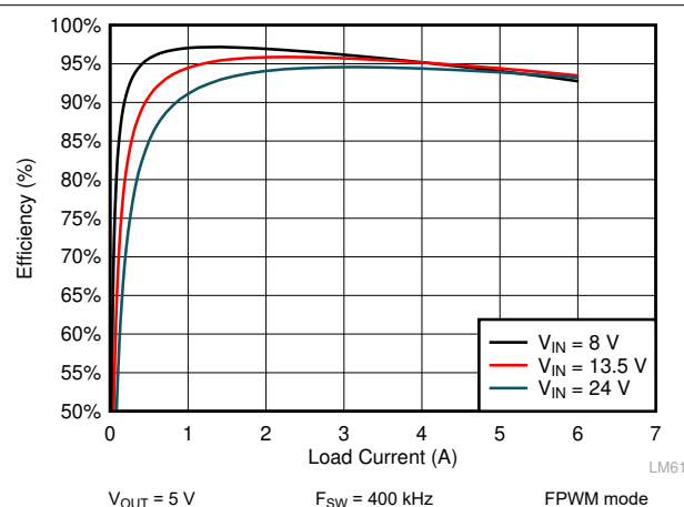
Figure 9-12. LM61460 Efficiency
