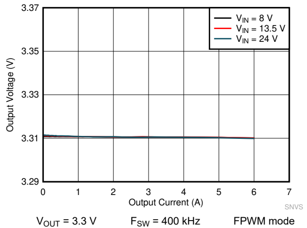
Figure 9-18. LM61460 Load and Line Regulation
