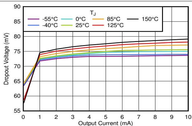
图 6-26. Dropout Voltage vs I_{OUT}
