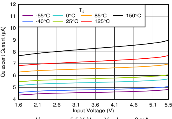
图 6-37. I_{GND} vs V_{IN} in the Dropout Region
