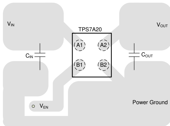
图 10-3. YCK Package (DSBGA) Typical Layout
