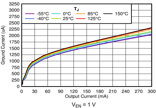
图 6-38. I_{GND} vs I_{OUT}
