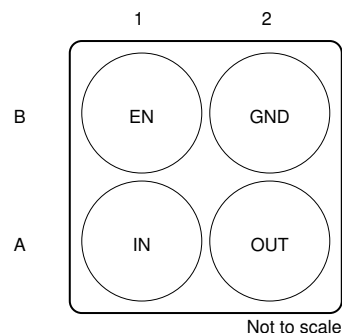
图 5-2. YCJ and YCK Packages (Preview), 4-Pin DSBGA, Bottom View
