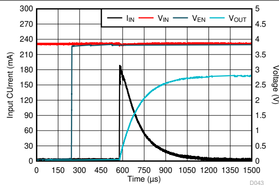
图 6-82. Start-Up
