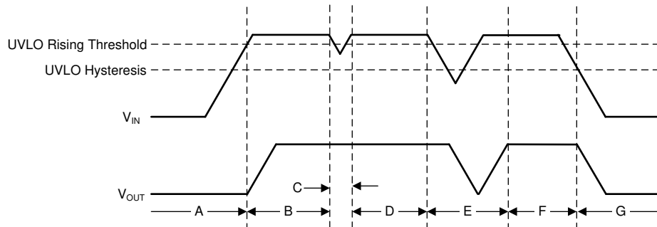
图 8-2. Typical UVLO Operation
