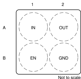
图 5-1. YCJ and YCK Packages (Preview), 4-Pin DSBGA, Top View
