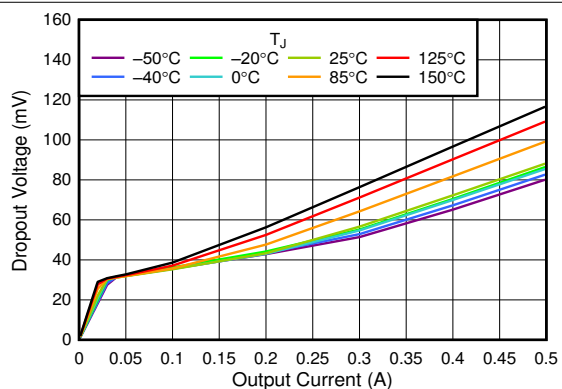
Figure 5-4. 3.3-V Dropout Voltage vs I_{OUT}
