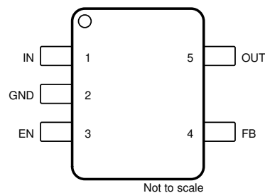
Figure 4-1. DRV Package, 6-Pin Adjustable WSON (Top View) Figure 4-2. DBV Package, 5-Pin Adjustable SOT-23 (Top View)
