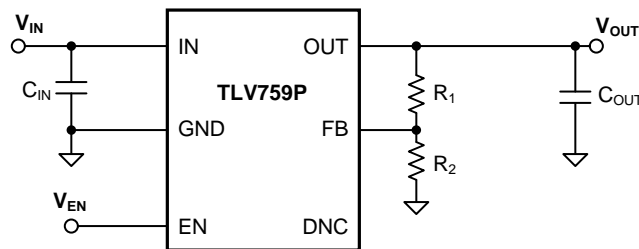
Figure 40. Adjustable Operation
