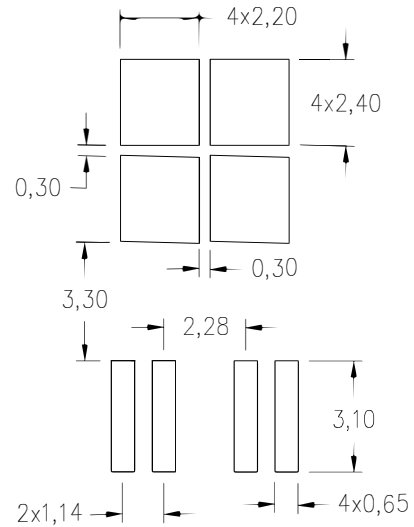
Stencil Openings Based on a stencil thickness of .127mm (.005inch).
