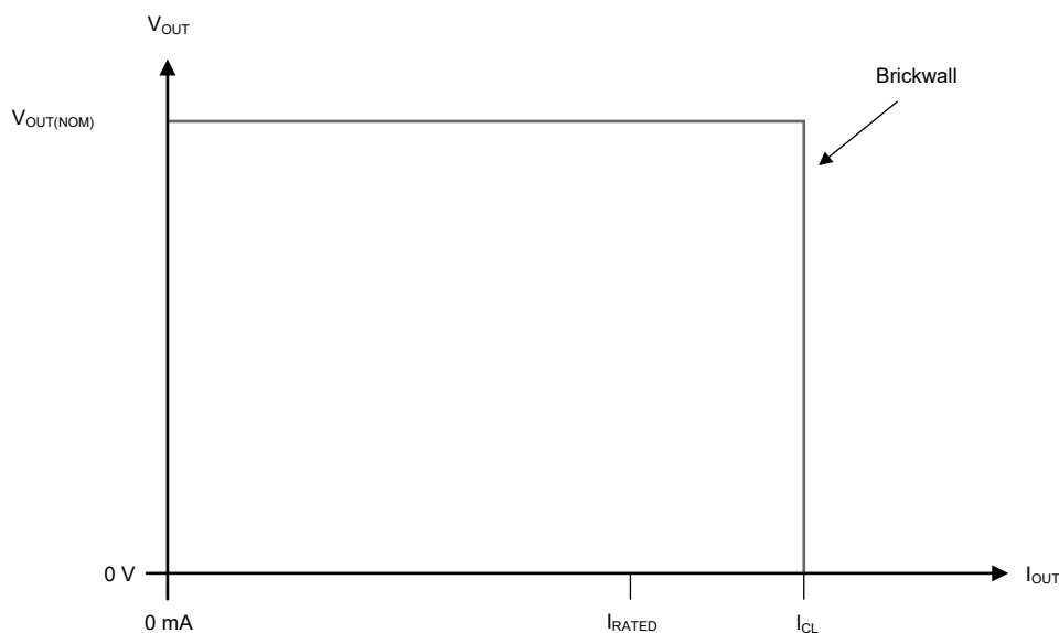
Figure 7-5. Current Limit
