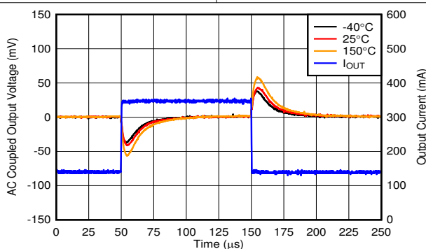
Figure 8-10. Transient Response
