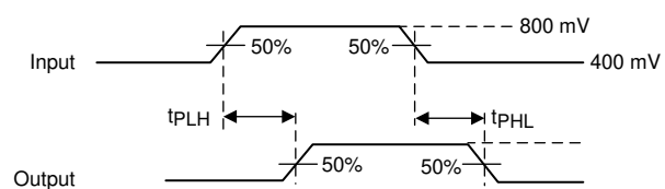
Figure 6-5. Propagation Delay
