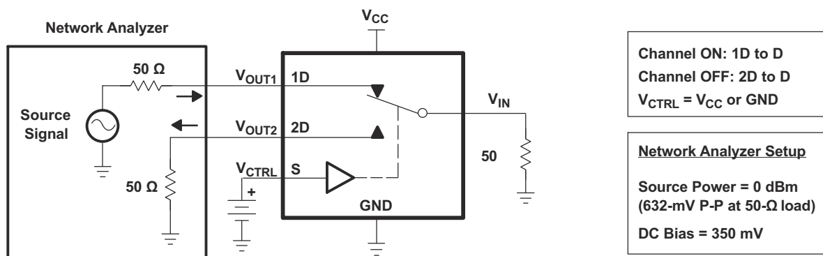
Figure 6-3. Crosstalk ( X_{TALK} )
