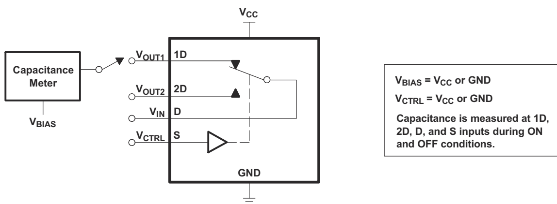
Figure 6-9. Capacitance
