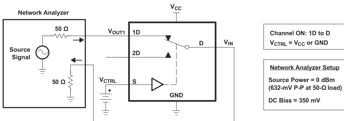
Figure 6-4. Bandwidth (BW)
