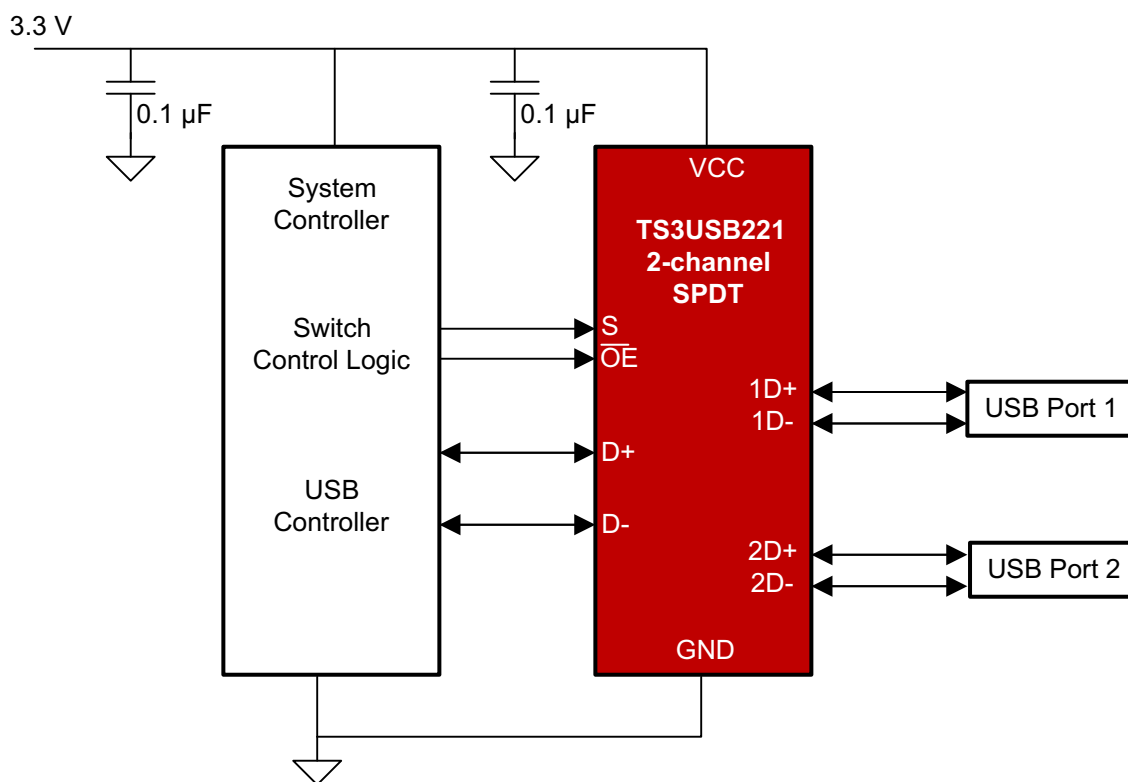
Figure 8-1. Simplified Schematic
