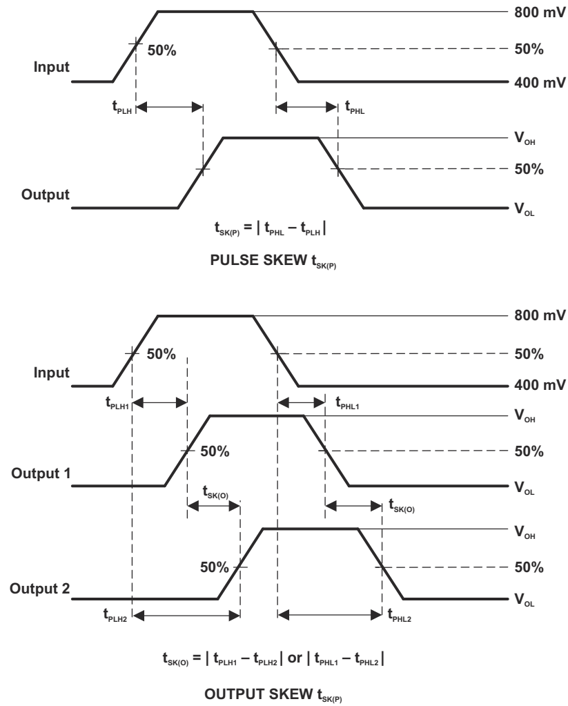
Figure 6-6. Skew Test
