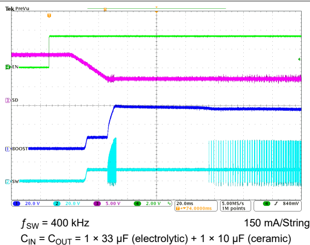
Figure 8-4. Typical Start-Up
