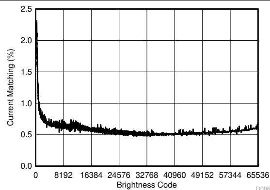
Figure 5-7. Current Matching
