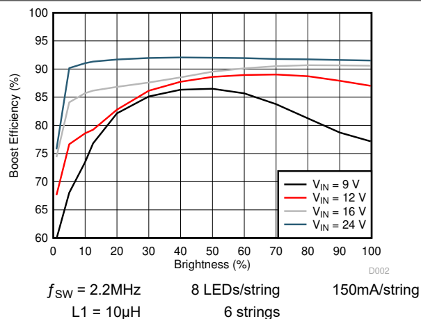
Figure 5-3. Boost Efficiency
