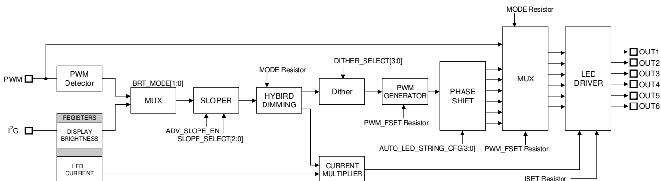
Figure 6-9. LP8866-Q1 Brightness Path Diagram
