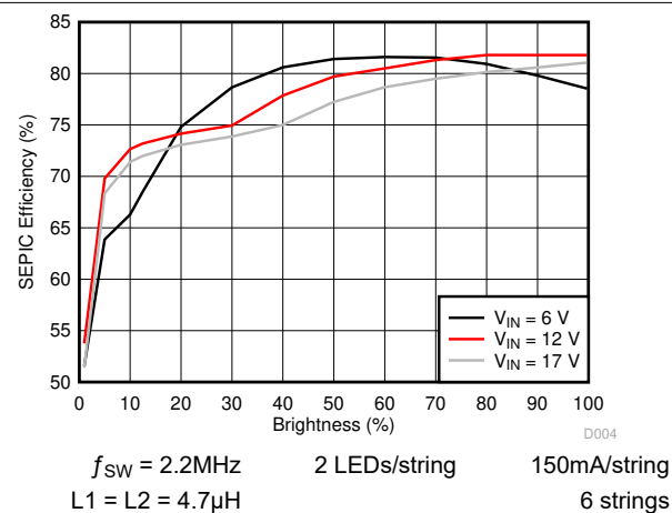
Figure 5-5. SEPIC Efficiency
