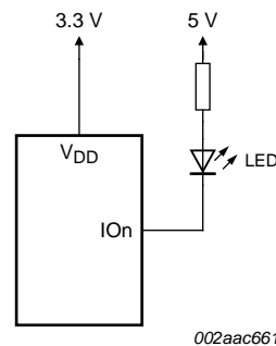
Fig 11. Device supplied by a lower voltage
