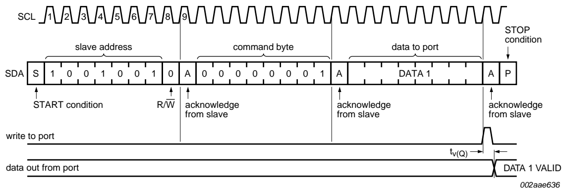
Fig 5. Write to output port register
