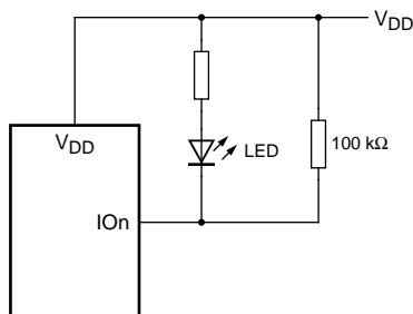
Fig 10. High value resistor in parallel with the LED
