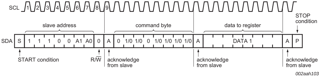
Fig 8. Write to Configuration or Polarity inversion registers
