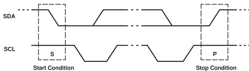
Figure 8-3. Definition Of Start And Stop Conditions
