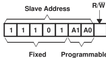
Figure 8-6. Pca9539 Address
