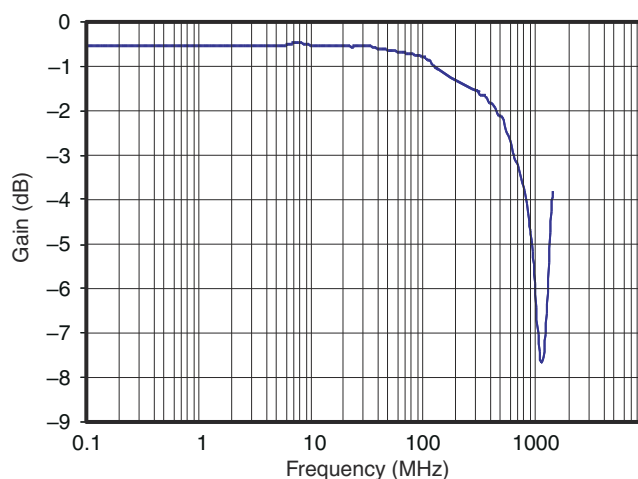
Figure 10-2. 3-dB Bandwidth
