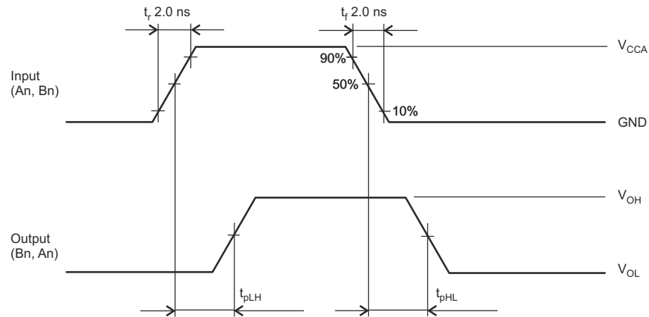
Figure 8-3. t_{PLH} , t_{PHL}
