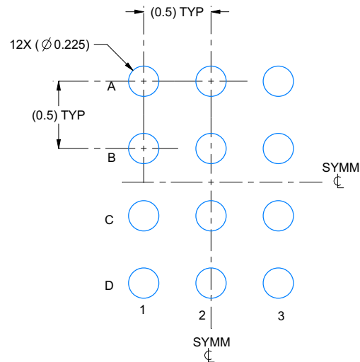
LAND PATTERN EXAMPLE SCALE:30X
