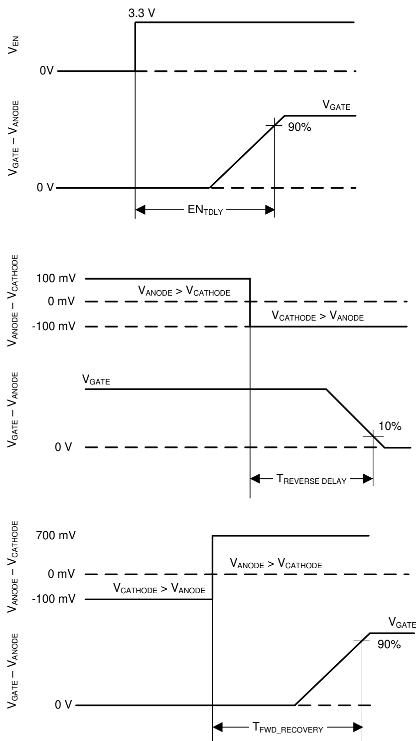
Figure 8-1. Timing Waveforms
