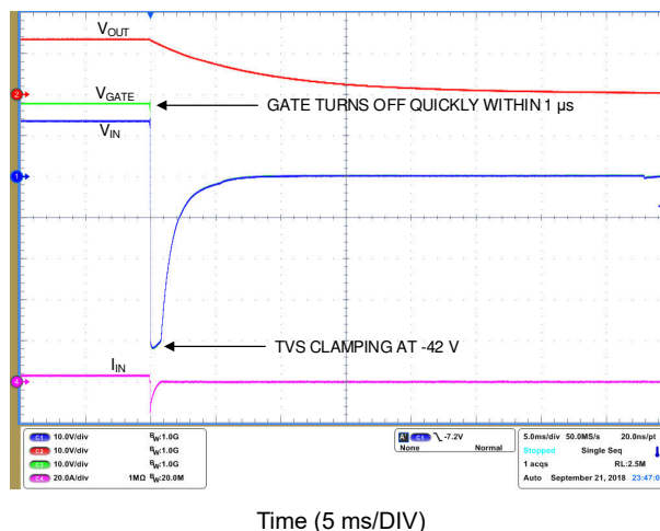
Figure 10-5. Response to ISO 7637-2 Pulse 1
