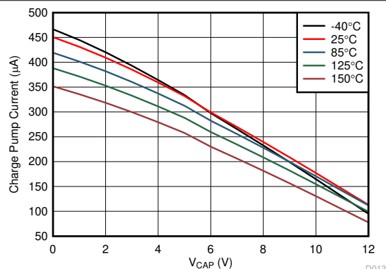
Figure 7-6. Charge Pump V-I Characteristics at V_ANODE &gt;= 12 V
