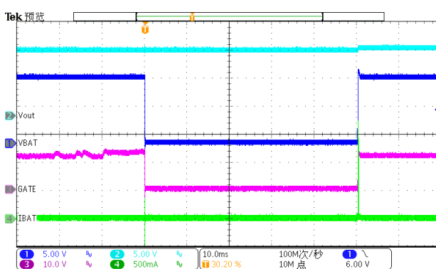
Figure 19. Input Micro-Short
