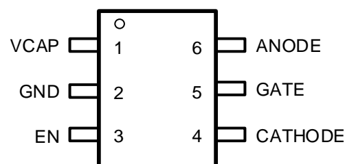
Figure 1. 6-Lead Plastic SOT23-6L
