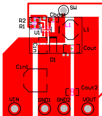
Figure 15. Layout
