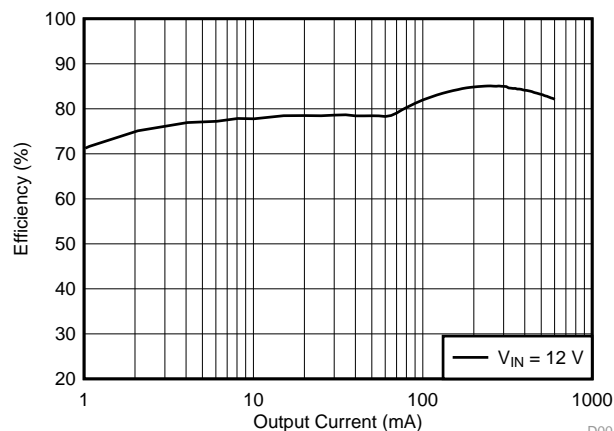
Efficiency vs Output Current ( f_{SW} = 2.1 MHz, V_{OUT} = 3.3 V)
