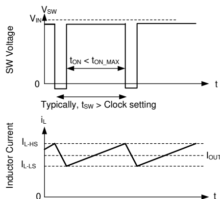
Figure 9-12. Current Limit Waveforms
