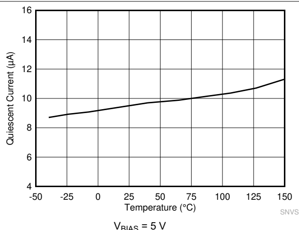
Figure 8-1. Non-Switching Input Supply Current
