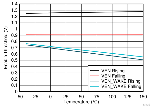
Figure 8-7. Enable Thresholds
