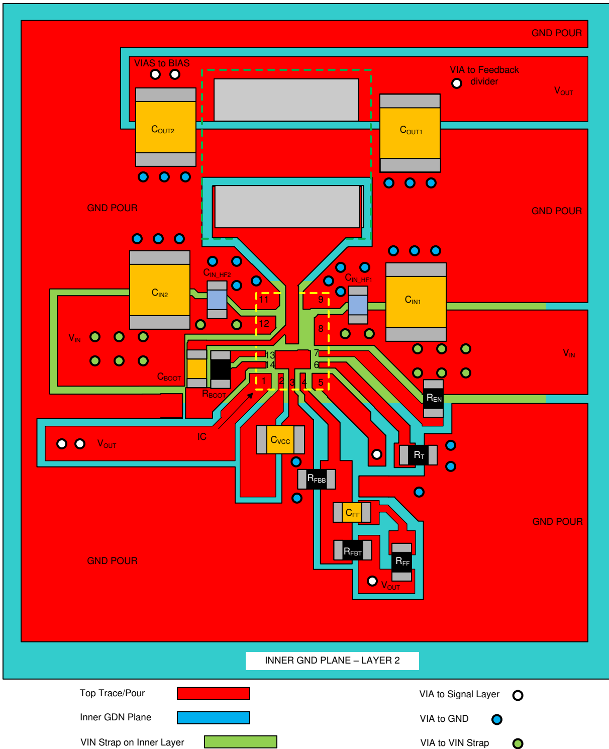
Figure 12-2. Layout Example
