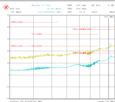
Figure 10-35. Conducted EMI versus CISPR25 Limits (Yellow: Peak Signal, Blue: Average Signal)
