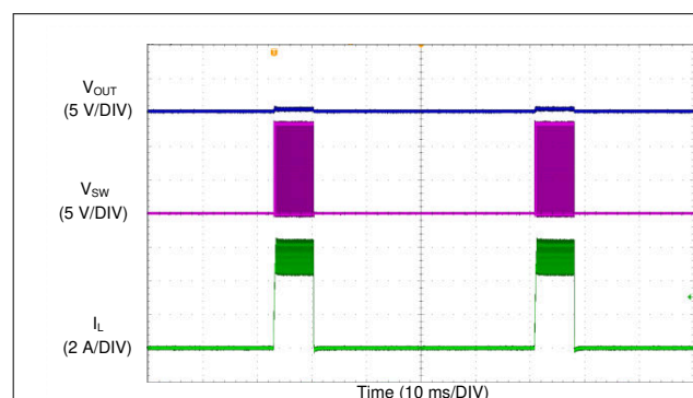
Figure 9-13. Inductor Current Bursts During Hiccup
