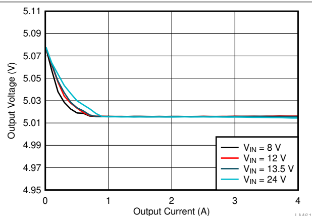
Figure 10-13. LM61440-Q1 Load and Line Regulation
