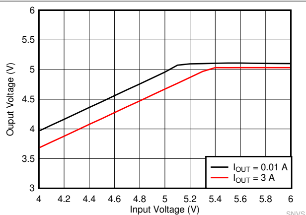
Figure 10-18. LM61440-Q1 Dropout Curve
