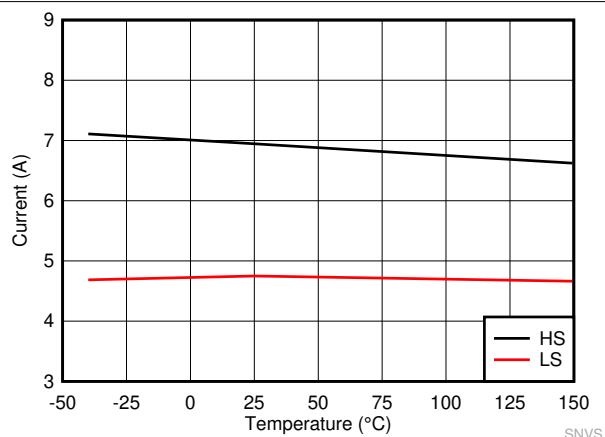
Figure 8-4. LM61440-Q1 High-side and Low-side Current Limits
