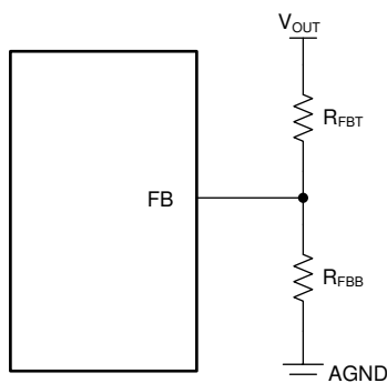
Figure 9-11. Setting Output Voltage of Adjustable Versions
