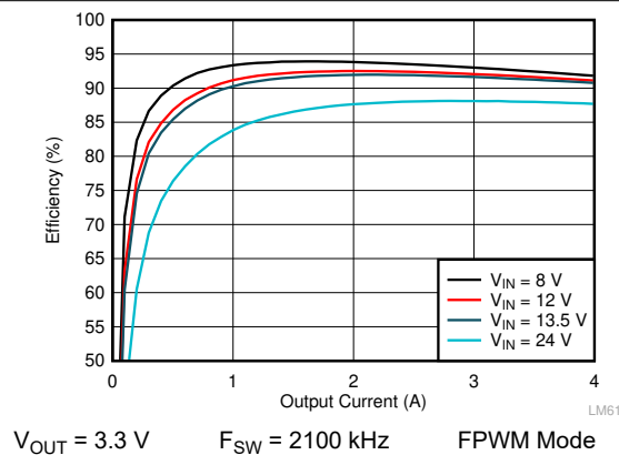
Figure 10-6. LM61440-Q1 Efficiency
