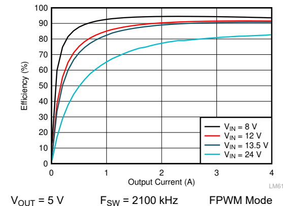
Figure 10-8. LM61440-Q1 Efficiency
