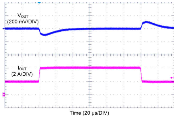
Figure 10-31. LM61440-Q1 Load Transient
