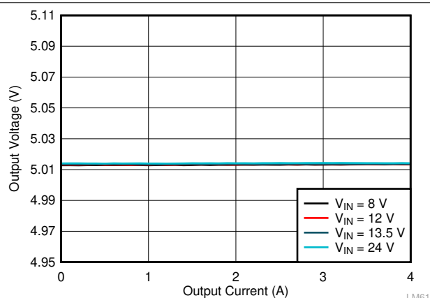
Figure 10-12. LM61440-Q1 Load and Line Regulation
