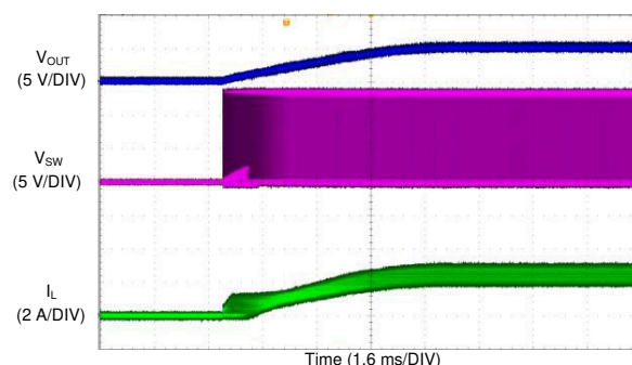
Figure 9-14. Short Circuit Recovery
