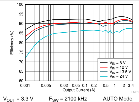
Figure 10-5. LM61440-Q1 Efficiency
