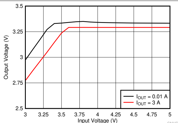
Figure 10-17. LM61440-Q1 Dropout Curve
