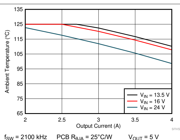
Figure 10-3. Maximum Ambient Temperature versus Output Current
