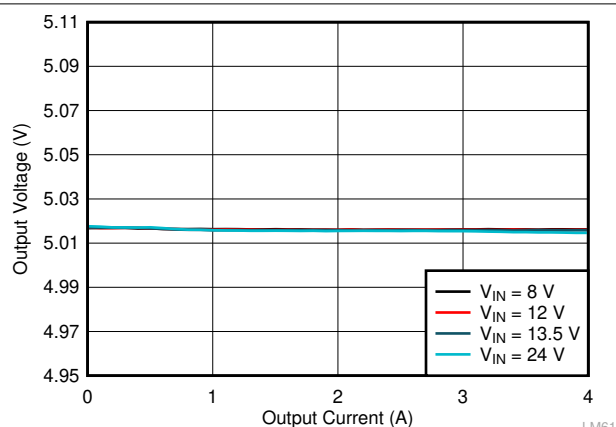
Figure 10-14. LM61440-Q1 Load and Line Regulation
