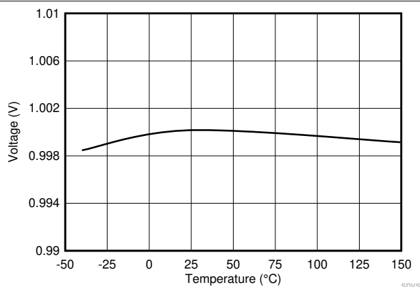
Figure 8-3. Feedback Voltage
