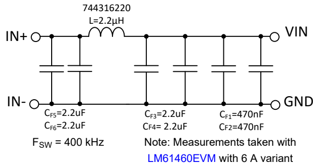
Figure 10-41. Recommended Input EMI Filter
