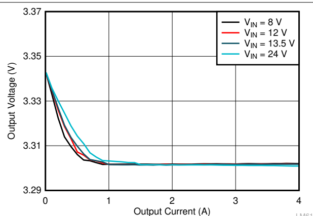
Figure 10-11. LM61440-Q1 Load and Line Regulation
