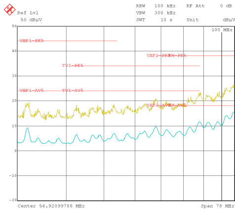
Figure 10-43. Conducted EMI versus CISPR25 Limits (Yellow: Peak Signal, Blue: Average Signal)
