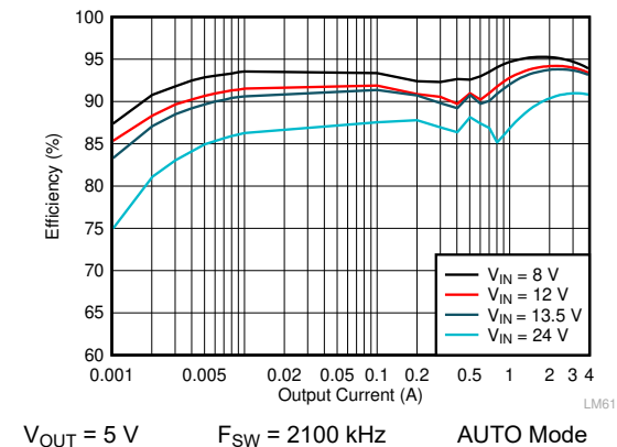
Figure 10-7. LM61440-Q1 Efficiency
