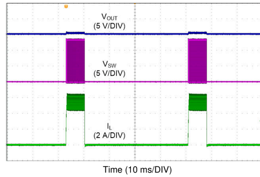
Figure 10-30. LM61440-Q1 Short Circuit Performance
