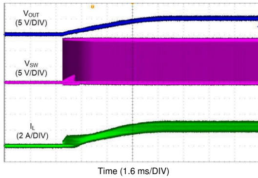
Figure 10-29. LM61440-Q1 Short Circuit Recovery
