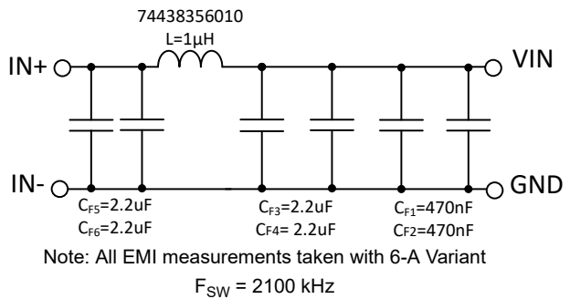
Figure 10-44. Recommended Input EMI Filter
