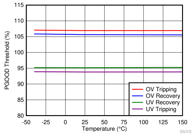
Figure 8-8. PGOOD Thresholds
