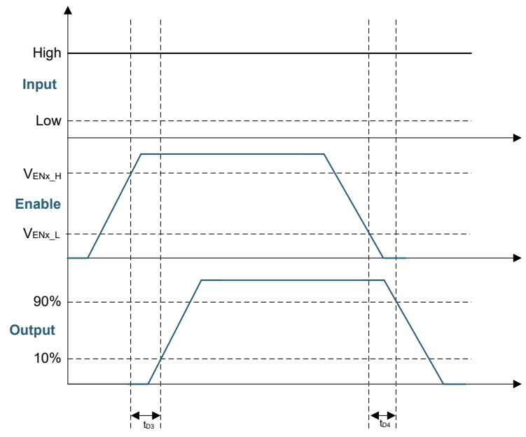
Figure 6-1. Enable Function
