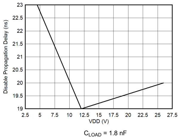
Figure 6-21. Enable to Output Falling Propagation Delay
