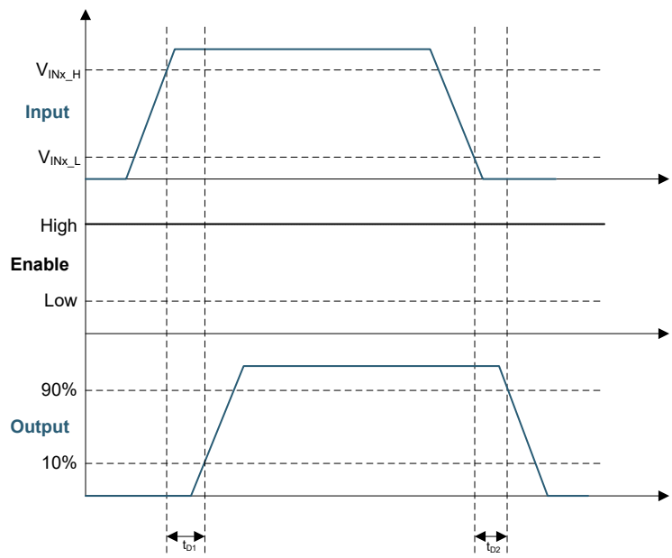
Figure 6-2. Input-Output Operation
