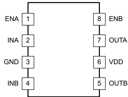
Figure 5-1. D and DGN Packages 8-Pin SOIC and HVSSOP-PowerPAD Top View
