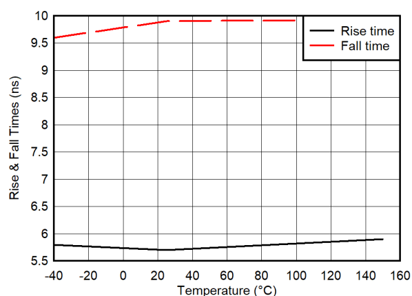
Figure 6-16. Output Rise and Fall Time vs Temperature
