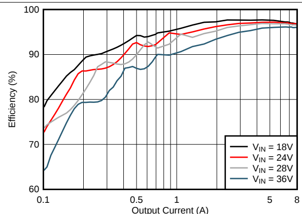
Figure 2. Efficiency vs Load, DCM
