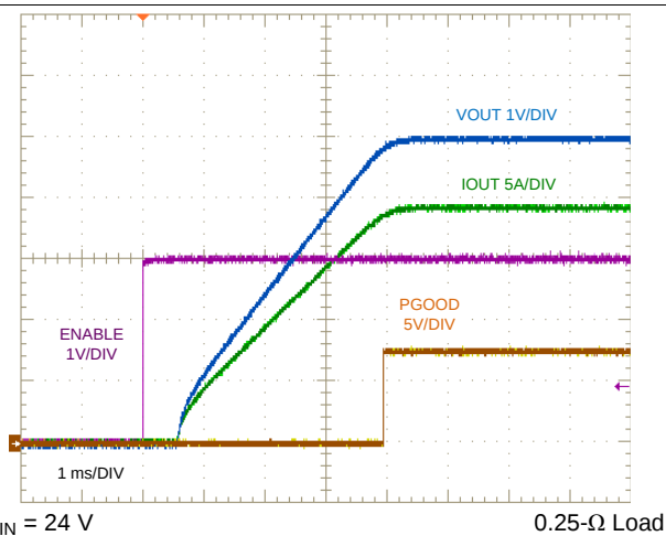
Figure 51. ENABLE ON, 20-A Resistive Load
