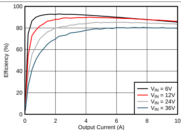
Figure 3. Efficiency vs Load, CCM
