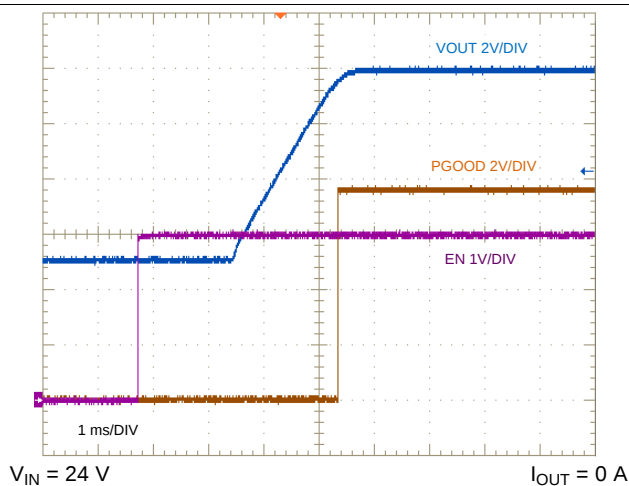
Figure 64. Pre-Biased Start-Up
