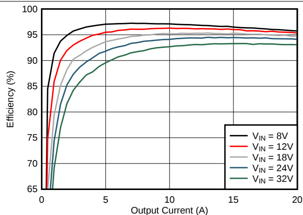
Figure 1. Efficiency vs Load, CCM
