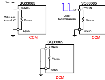
Fig 9. CCM&DCM Selection
