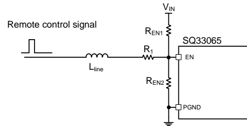
Fig 6. Remote Control Circuit
