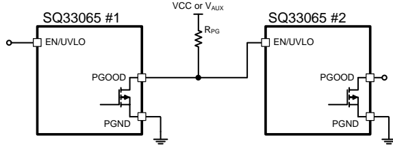
Fig 12. PGOOD Controlling EN/UVLO Type-III Voltage Mode Control (COMP&FB)
