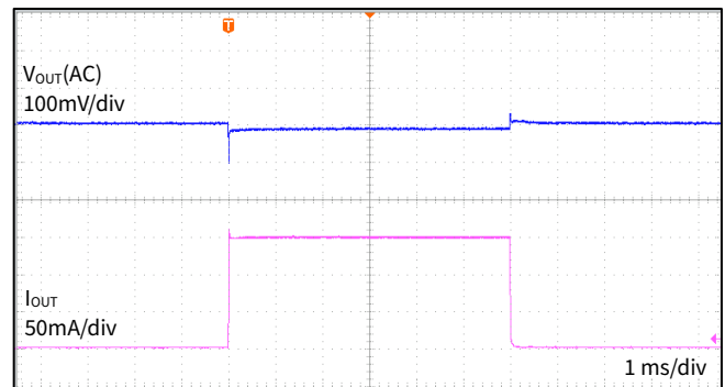
Figure 14 Load Transient
