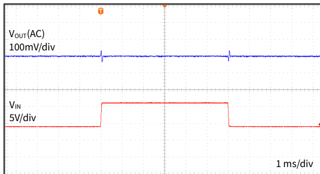
Figure 13 Line Transient
