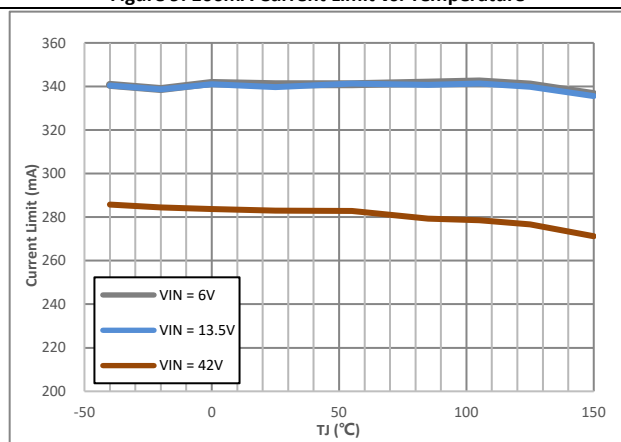
LN20542Q1, Fixed V_{OUT} = 5V , Measured at V_{OUT} short
