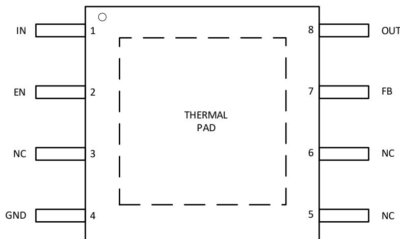
MSOP-EP8
