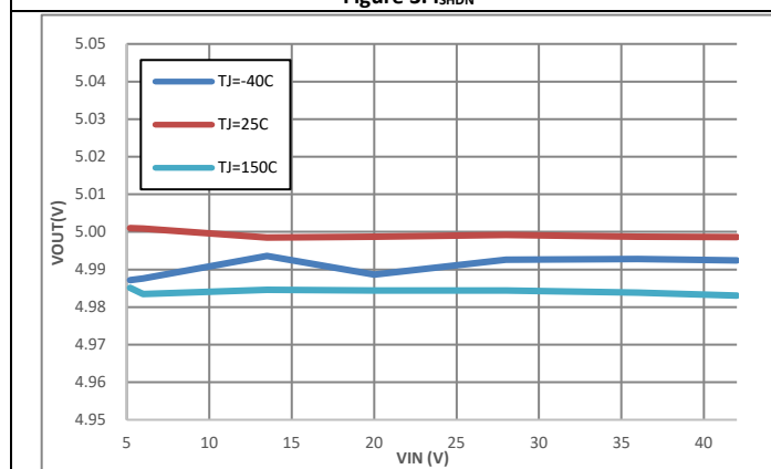
LN20042Q1, Adjustable V_{OUT} = 5\text{V} , I_{OUT} = 1\text{mA}
