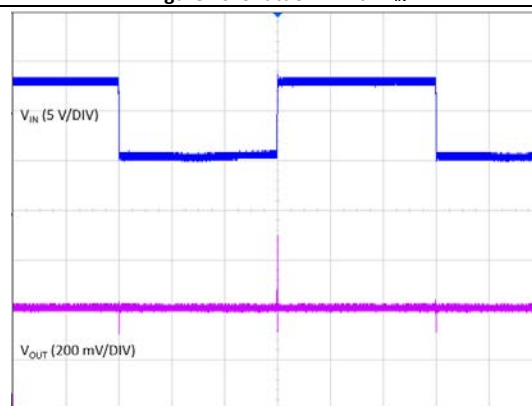
Figure 16. Shutdown with V_{\text{IN}}
