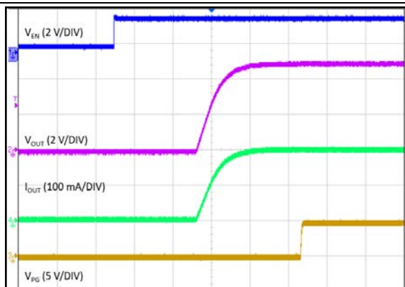
Figure 13. Startup with EN
