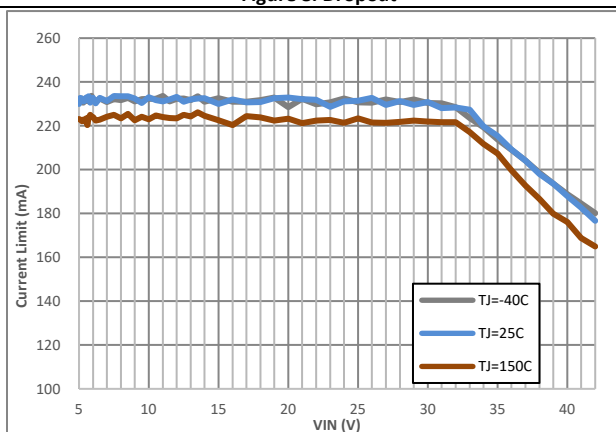
LN20041Q1, Adjustable V_{OUT} = 5V , Measured at V_{OUT} short
