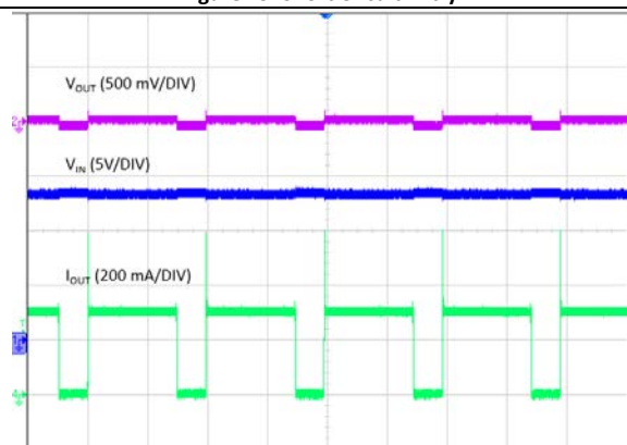
Time (5ms/DIV) LN20042Q1, Adjustable V_{OUT} = 5\text{V} , V_{IN} = 13.5\text{V}
