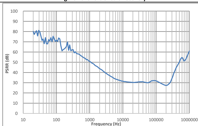
LN20042Q1, Adjustable V_{OUT} = 5\text{V} , C_{IN} = 100\text{pF} , V_{IN} = 6\text{V} , I_{OUT} = 10\text{mA}
