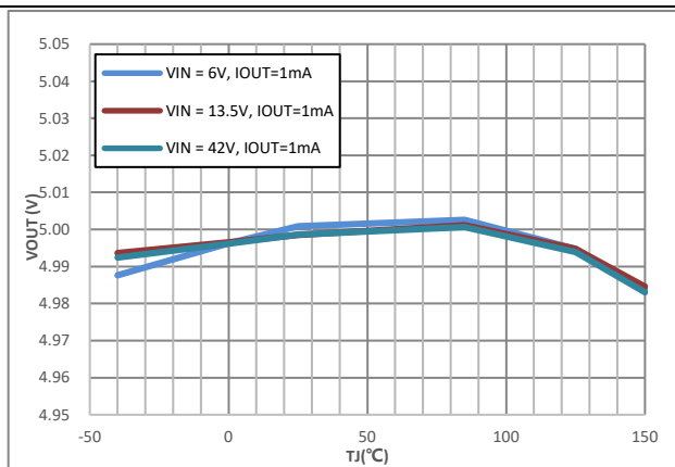
LN20042Q1, Adjustable V_{OUT} = 5V , I_{OUT} = 1mA
