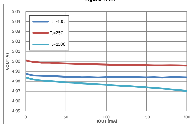
LN20042Q1, Adjustable V_{OUT} = 5\text{V} , V_{IN} = 13.5\text{V}
