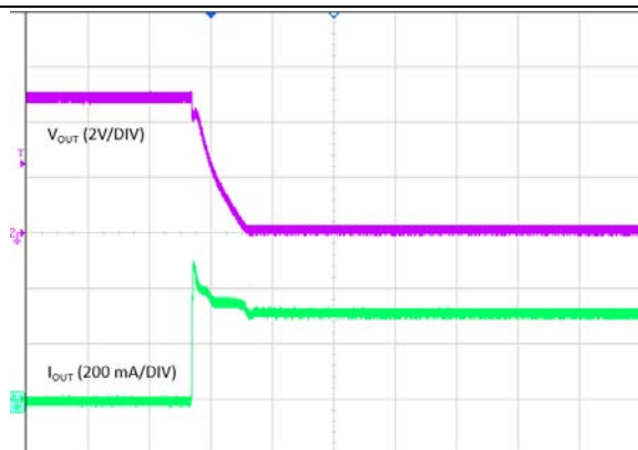
Time (200μs/DIV) LN20042Q1, Adjustable V_{OUT} = 5\text{V} , V_{IN} = 13.5\text{V}
