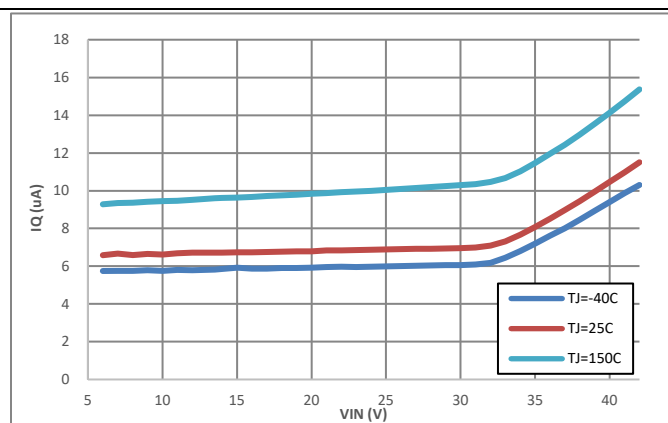
LN20442Q1, Fixed V_{OUT} = 5\text{V} , With PG, No load
