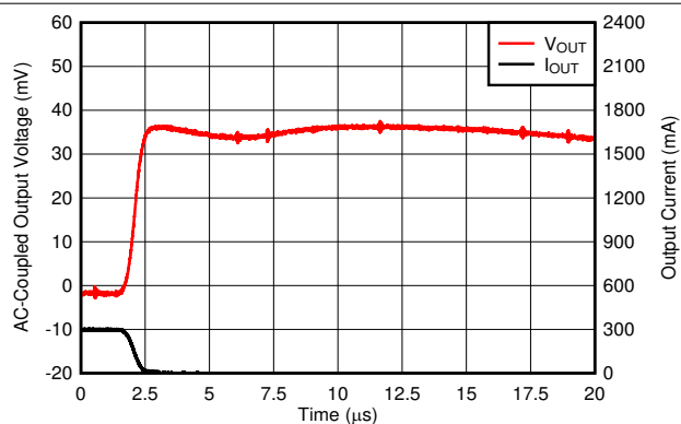
Figure 6-20. I_{OUT} Transient From 300 mA to 1 mA
