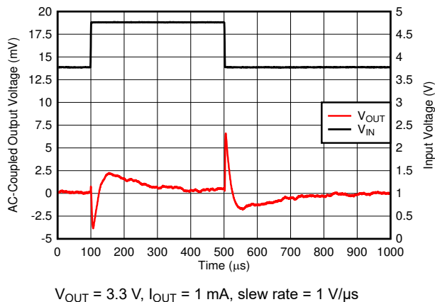
Figure 6-16. Line Transient
