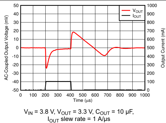
Figure 8-9. I_{\text{OUT}} Transient From 1 mA to 100 mA
