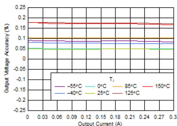
Output Accuracy vs I_{OUT} for 5.0 V
