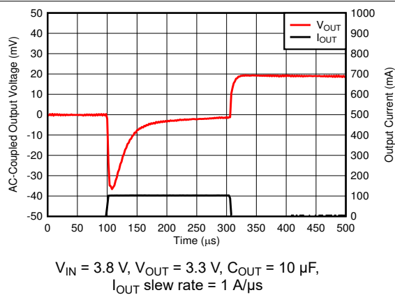
Figure 8-8. I_{\text{OUT}} Transient From 0 mA to 100 mA
