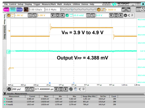
Figure 12. Line Transient
